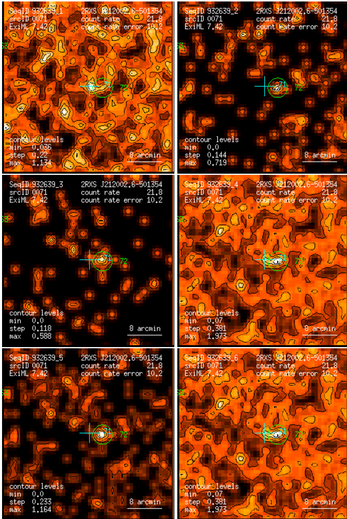
Figure 71: RASS 932639: detection 0071: band rate images, Gaussian filter: (1) PSPC channels 11 – 41, (2) 52 – 90, (3) 91 – 201, (4) 11 – 235, (5) 52 – 201, (6) 11 – 201. Broad band rates in counts/ks. Band rate contour levels in counts/ks/arcmin 2 .
