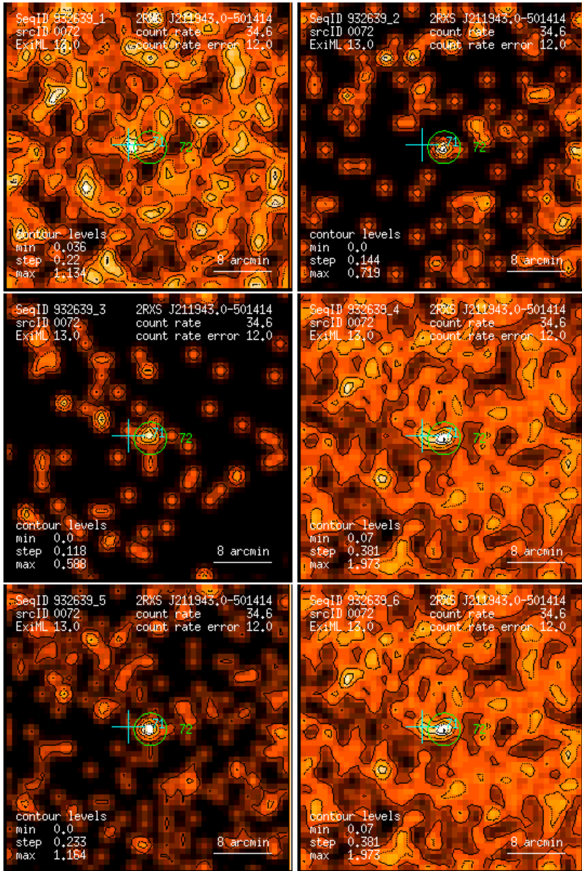
Figure 72: RASS 932639: detection 0072: band rate images, Gaussian filter: (1) PSPC channels 11 – 41, (2) 52 – 90, (3) 91 – 201, (4) 11 – 235, (5) 52 – 201, (6) 11 – 201. Broad band rates in counts/ks. Band rate contour levels in counts/ks/arcmin 2 .
