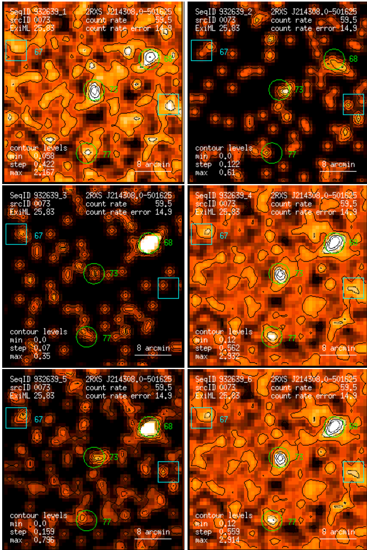
Figure 73: RASS 932639: detection 0073: band rate images, Gaussian filter: (1) PSPC channels 11 – 41, (2) 52 – 90, (3) 91 – 201, (4) 11 – 235, (5) 52 – 201, (6) 11 – 201. Broad band rates in counts/ks. Band rate contour levels in counts/ks/arcmin 2 .
