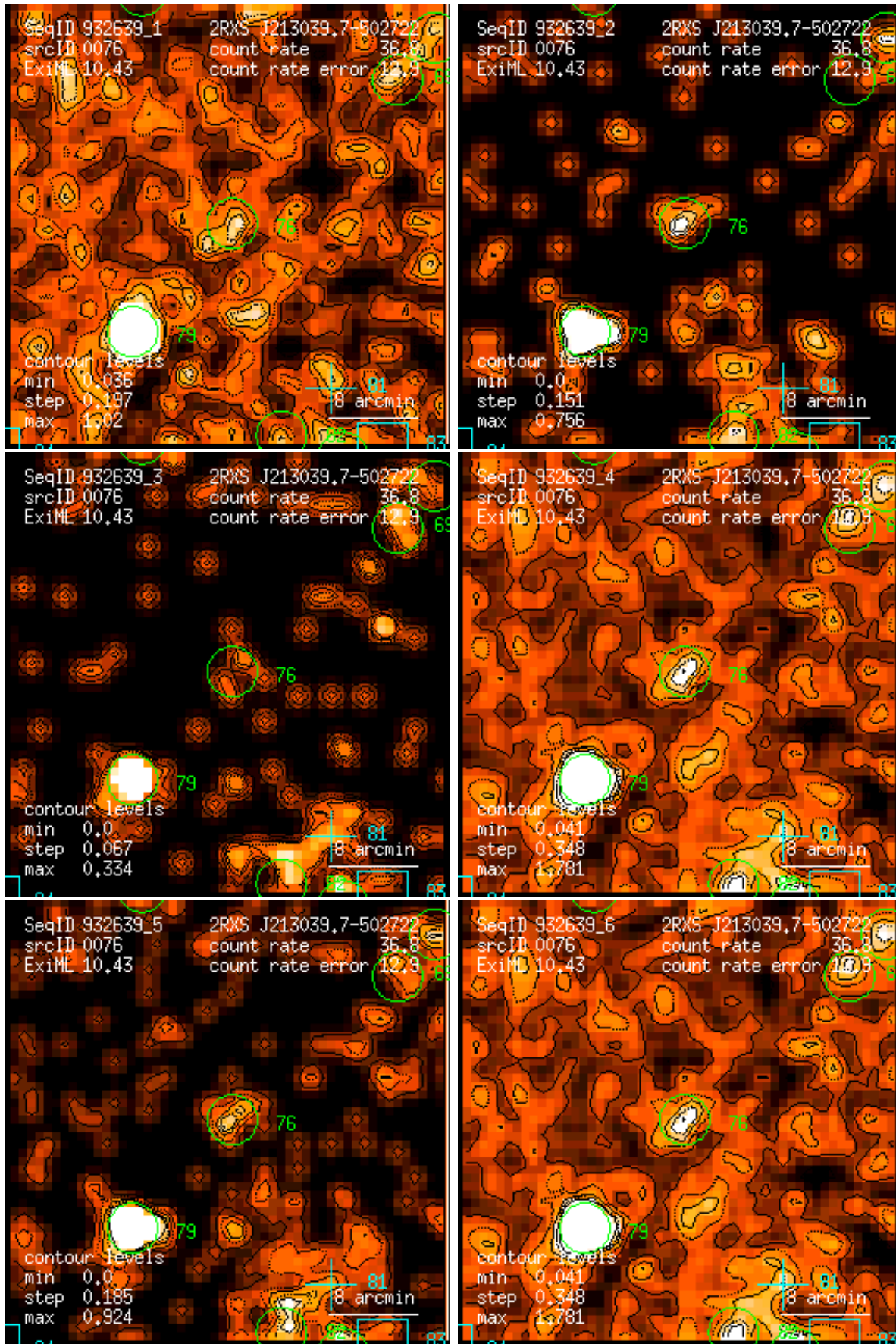
Figure 76: RASS 932639: detection 0076: band rate images, Gaussian filter: (1) PSPC channels 11 – 41, (2) 52 – 90, (3) 91 – 201, (4) 11 – 235, (5) 52 – 201, (6) 11 – 201. Broad band rates in counts/ks. Band rate contour levels in counts/ks/arcmin 2 .
