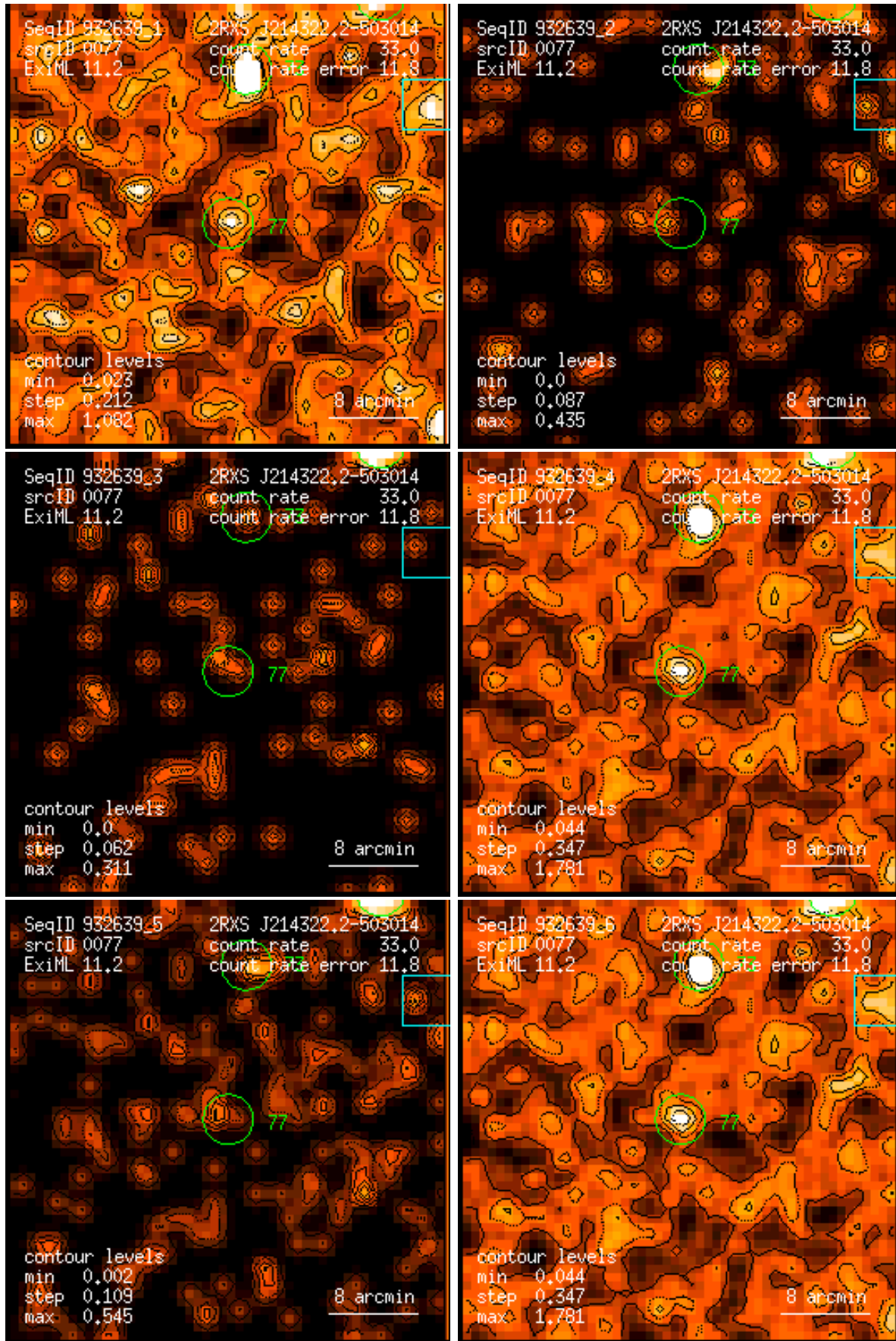
Figure 77: RASS 932639: detection 0077: band rate images, Gaussian filter: (1) PSPC channels 11 – 41, (2) 52 – 90, (3) 91 – 201, (4) 11 – 235, (5) 52 – 201, (6) 11 – 201. Broad band rates in counts/ks. Band rate contour levels in counts/ks/arcmin 2 .
