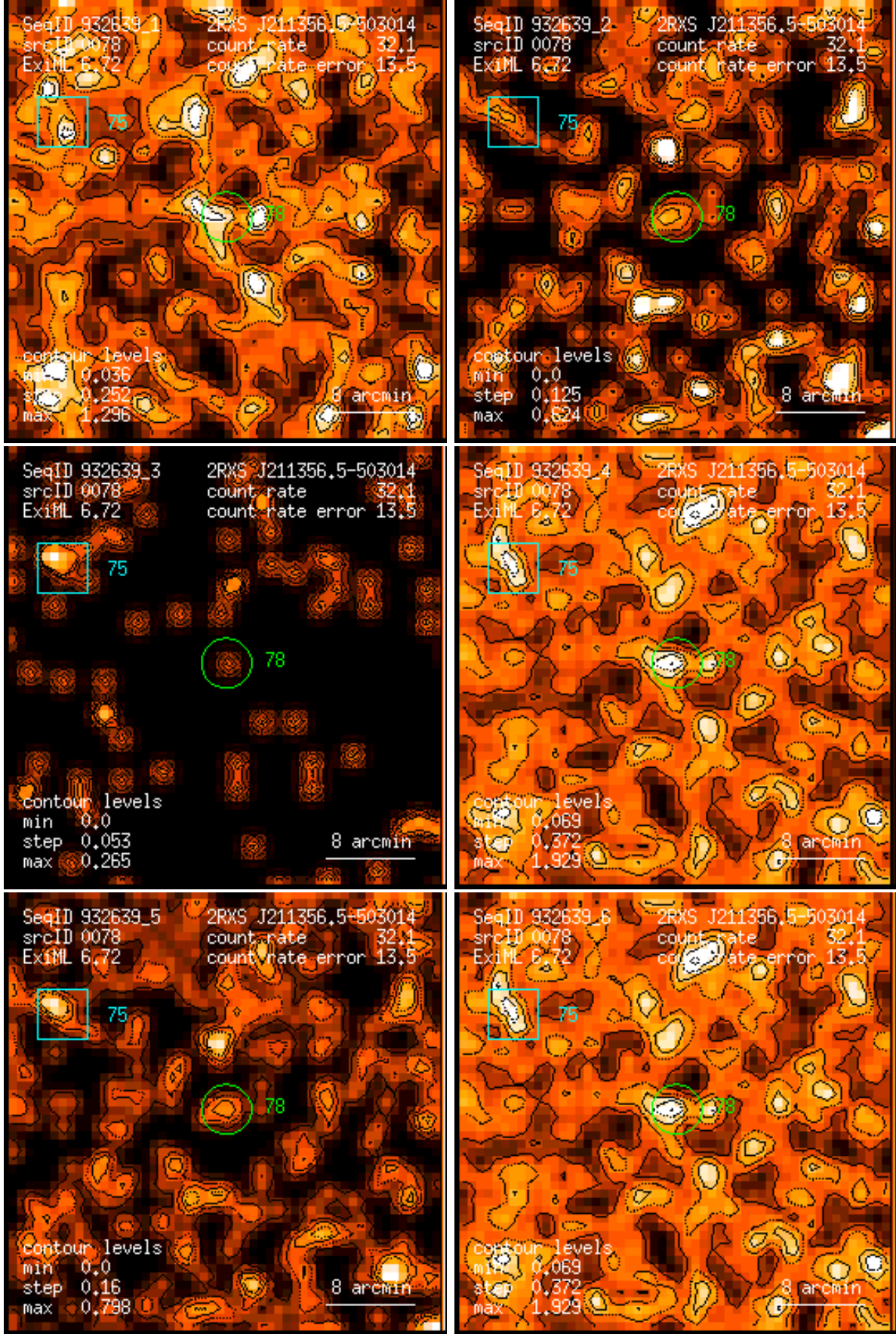
Figure 78: RASS 932639: detection 0078: band rate images, Gaussian filter: (1) PSPC channels 11 – 41, (2) 52 – 90, (3) 91 – 201, (4) 11 – 235, (5) 52 – 201, (6) 11 – 201. Broad band rates in counts/ks. Band rate contour levels in counts/ks/arcmin 2 .
