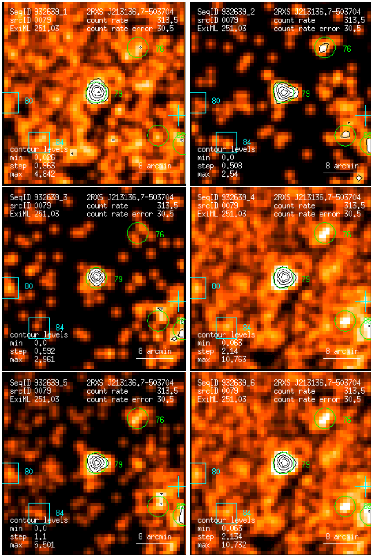
Figure 79: RASS 932639: detection 0079: band rate images, Gaussian filter: (1) PSPC channels 11 – 41, (2) 52 – 90, (3) 91 – 201, (4) 11 – 235, (5) 52 – 201, (6) 11 – 201. Broad band rates in counts/ks. Band rate contour levels in counts/ks/arcmin 2 .
