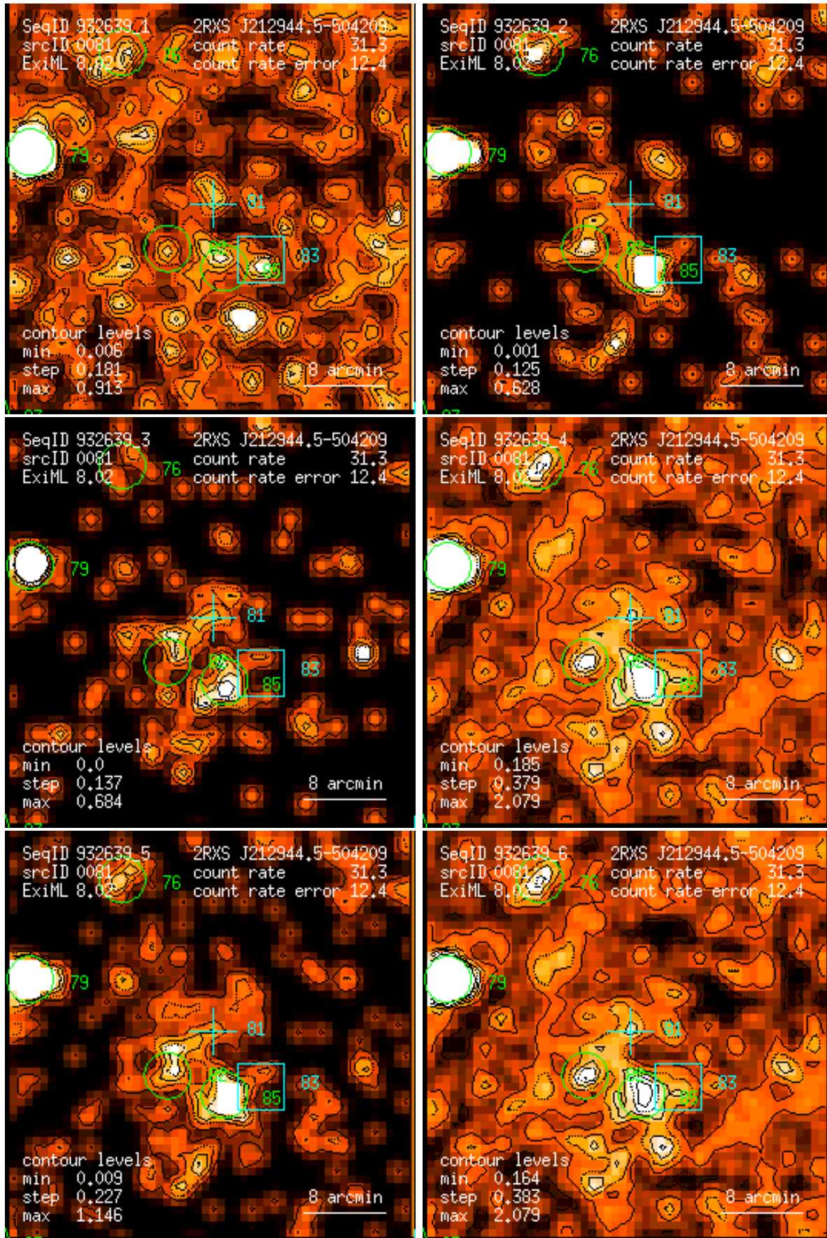
Figure 81: RASS 932639: detection 0081: band rate images, Gaussian filter: (1) PSPC channels 11 – 41, (2) 52 – 90, (3) 91 – 201, (4) 11 – 235, (5) 52 – 201, (6) 11 – 201. Broad band rates in counts/ks. Band rate contour levels in counts/ks/arcmin 2 .
