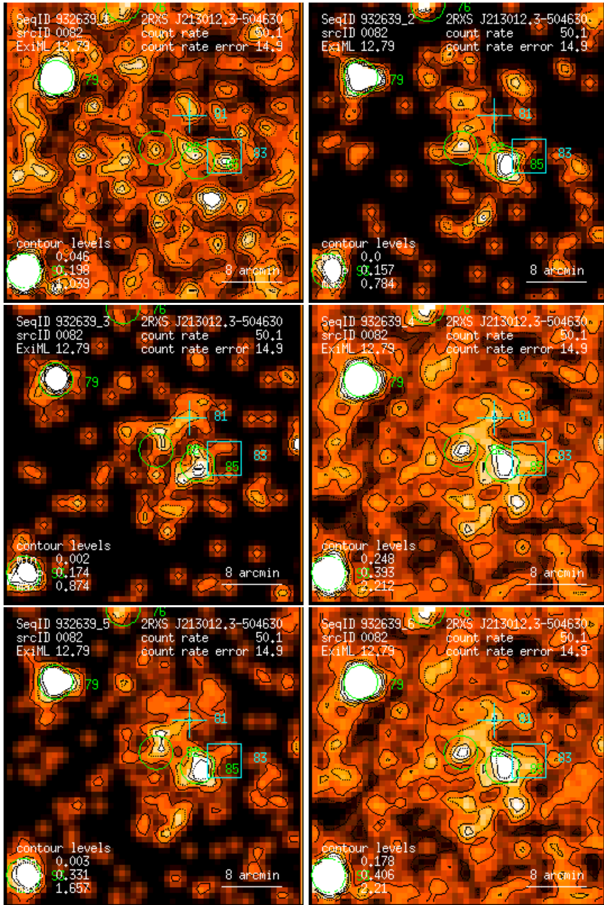
Figure 82: RASS 932639: detection 0082: band rate images, Gaussian filter: (1) PSPC channels 11 – 41, (2) 52 – 90, (3) 91 – 201, (4) 11 – 235, (5) 52 – 201, (6) 11 – 201. Broad band rates in counts/ks. Band rate contour levels in counts/ks/arcmin 2 .
