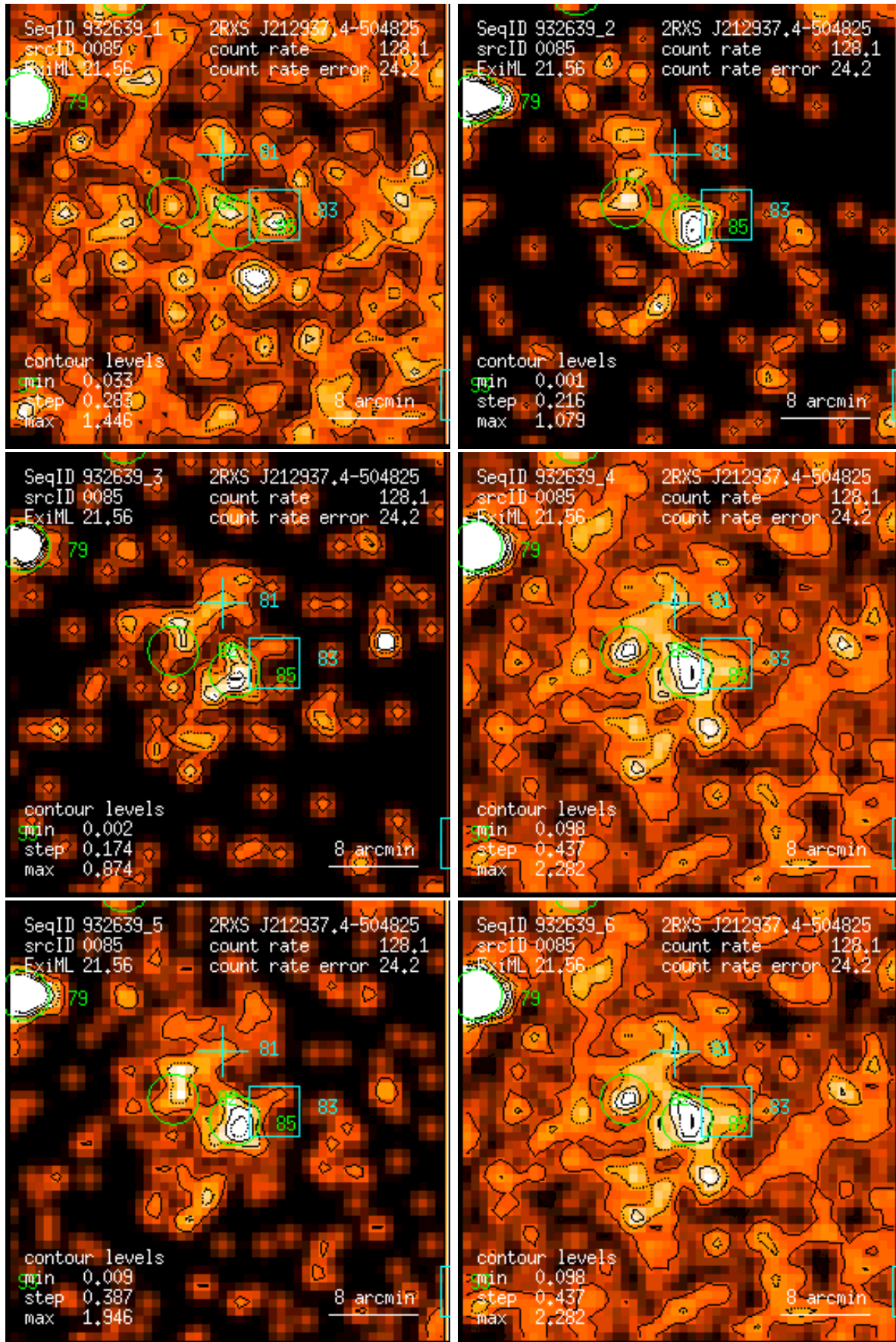
Figure 85: RASS 932639: detection 0085: band rate images, Gaussian filter: (1) PSPC channels 11 – 41, (2) 52 – 90, (3) 91 – 201, (4) 11 – 235, (5) 52 – 201, (6) 11 – 201. Broad band rates in counts/ks. Band rate contour levels in counts/ks/arcmin 2 .
