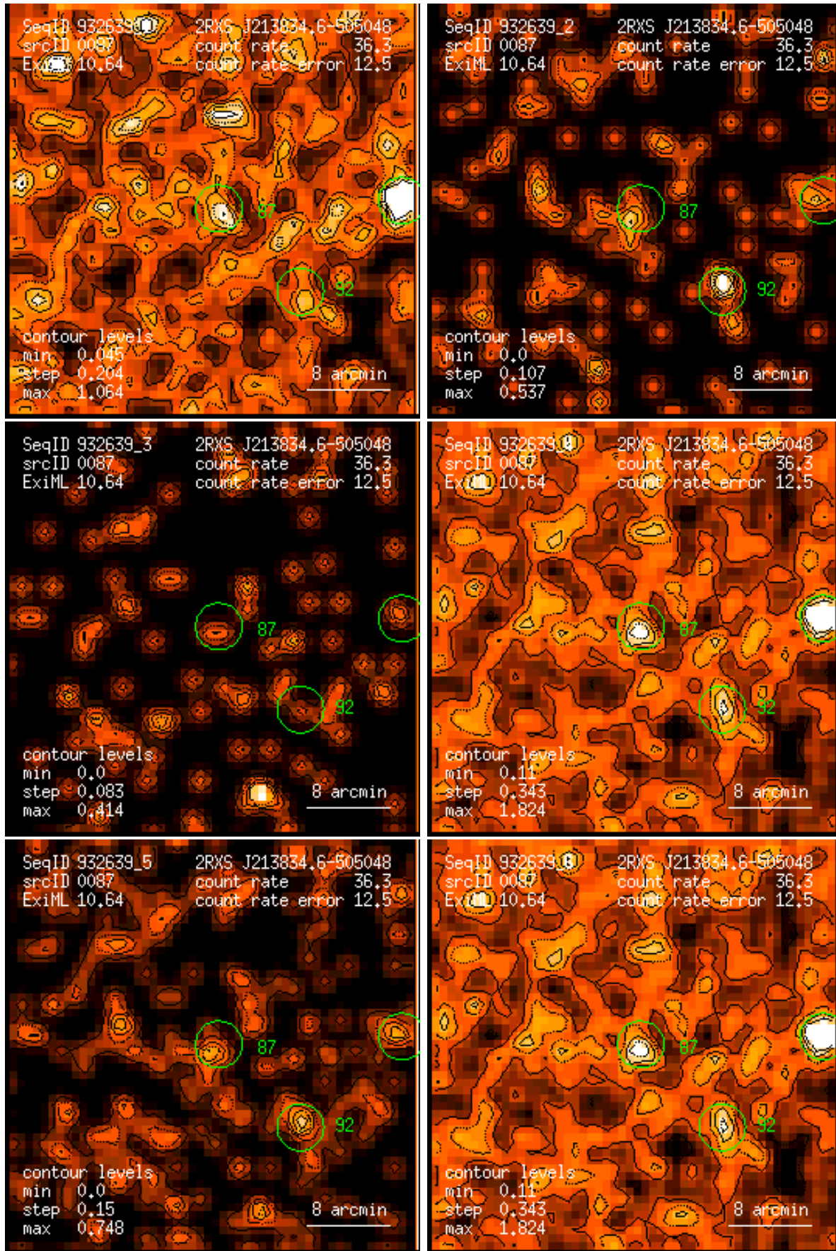
Figure 87: RASS 932639: detection 0087: band rate images, Gaussian filter: (1) PSPC channels 11 – 41, (2) 52 – 90, (3) 91 – 201, (4) 11 – 235, (5) 52 – 201, (6) 11 – 201. Broad band rates in counts/ks. Band rate contour levels in counts/ks/arcmin 2 .
