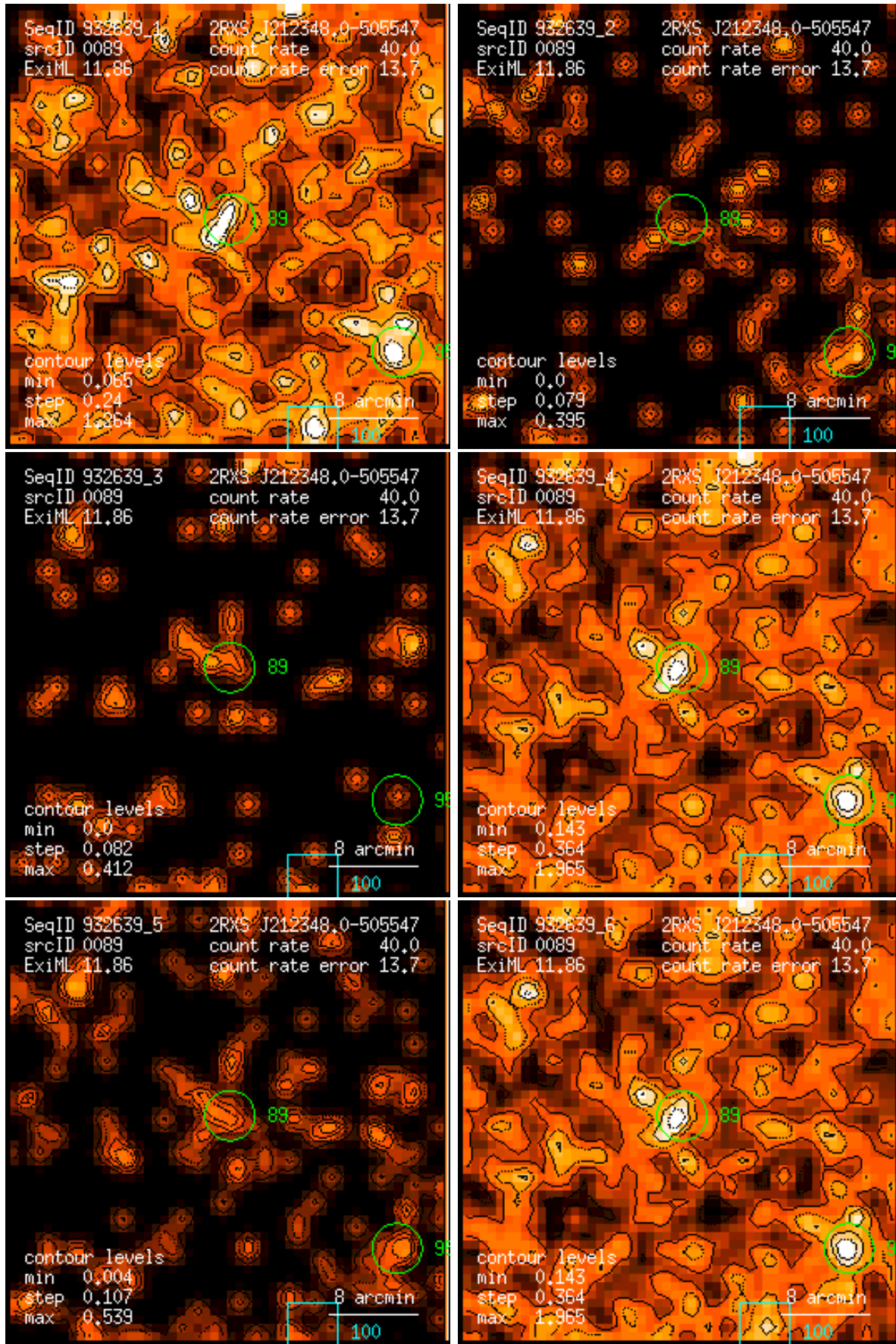
Figure 89: RASS 932639: detection 0089: band rate images, Gaussian filter: (1) PSPC channels 11 – 41, (2) 52 – 90, (3) 91 – 201, (4) 11 – 235, (5) 52 – 201, (6) 11 – 201. Broad band rates in counts/ks. Band rate contour levels in counts/ks/arcmin 2 .
