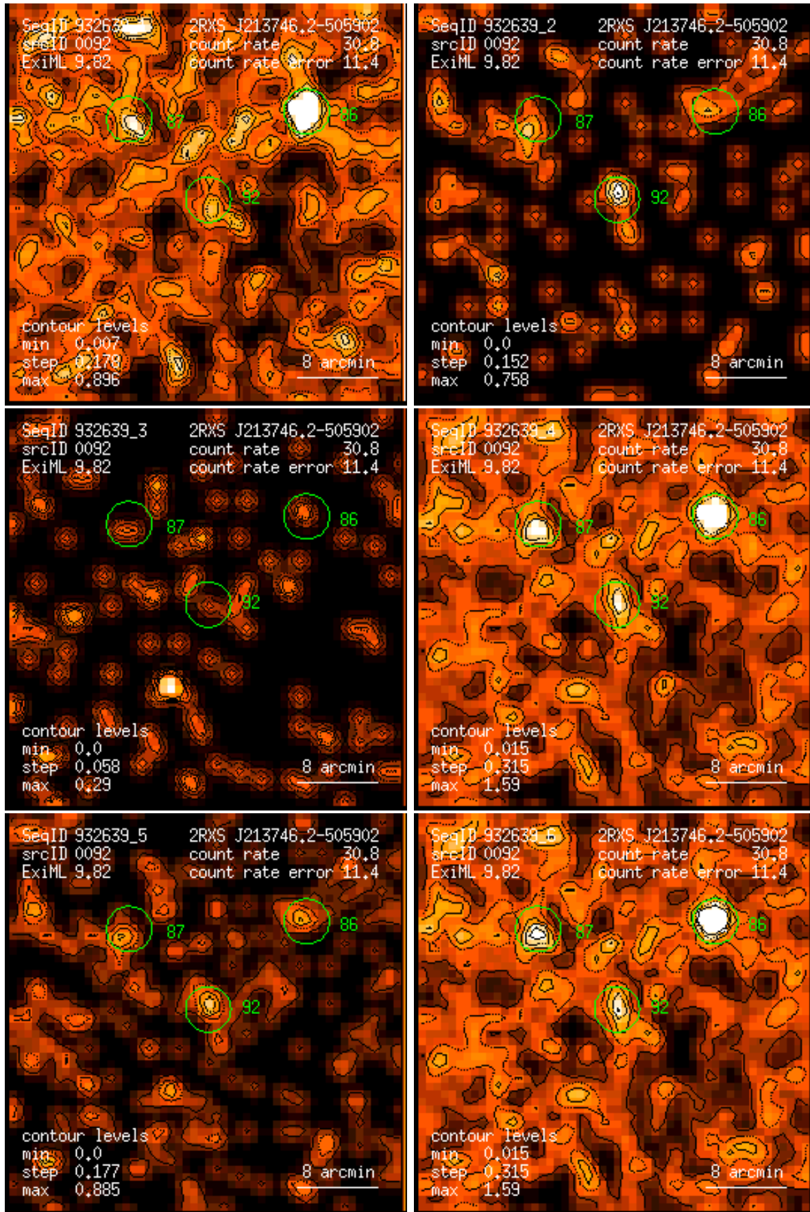
Figure 92: RASS 932639: detection 0092: band rate images, Gaussian filter: (1) PSPC channels 11 – 41, (2) 52 – 90, (3) 91 – 201, (4) 11 – 235, (5) 52 – 201, (6) 11 – 201. Broad band rates in counts/ks. Band rate contour levels in counts/ks/arcmin 2 .
