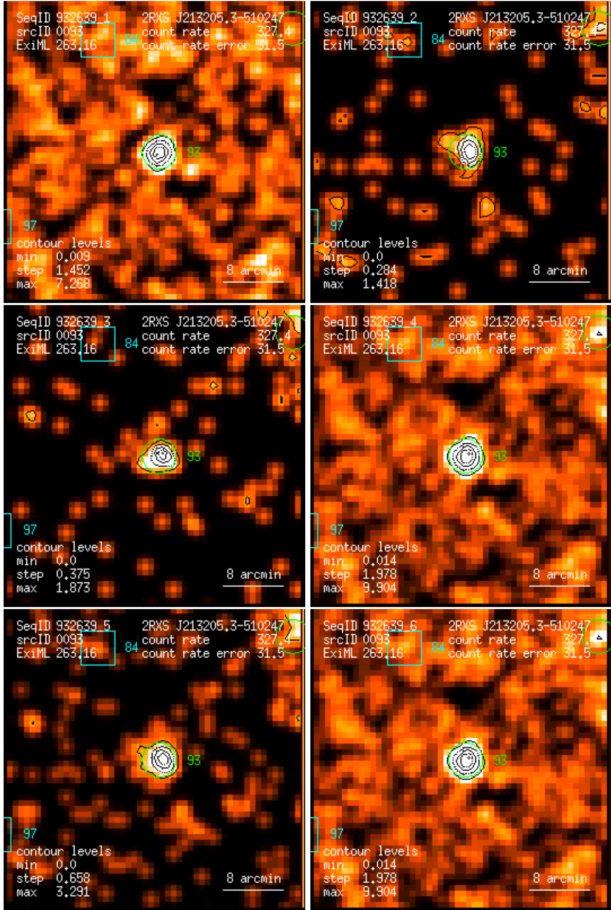
Figure 93: RASS 932639: detection 0093: band rate images, Gaussian filter: (1) PSPC channels 11 – 41, (2) 52 – 90, (3) 91 – 201, (4) 11 – 235, (5) 52 – 201, (6) 11 – 201. Broad band rates in counts/ks. Band rate contour levels in counts/ks/arcmin 2 .
