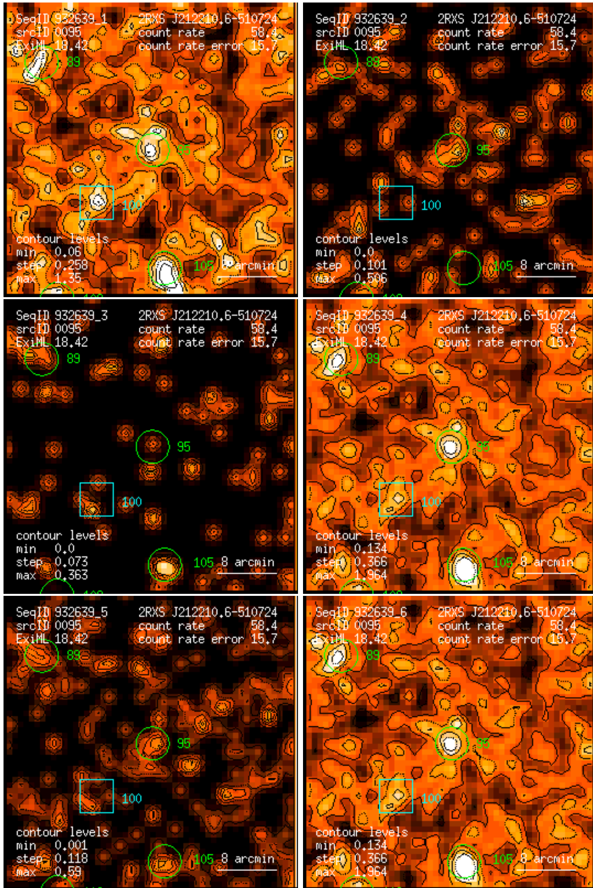
Figure 95: RASS 932639: detection 0095: band rate images, Gaussian filter: (1) PSPC channels 11 – 41, (2) 52 – 90, (3) 91 – 201, (4) 11 – 235, (5) 52 – 201, (6) 11 – 201. Broad band rates in counts/ks. Band rate contour levels in counts/ks/arcmin 2 .
