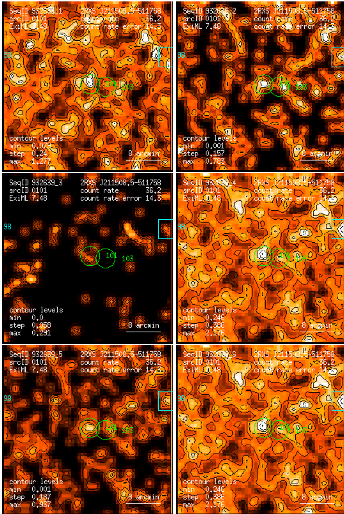
Figure 101: RASS 932639: detection 0101: band rate images, Gaussian filter: (1) PSPC channels 11 – 41, (2) 52 – 90, (3) 91 – 201, (4) 11 – 235, (5) 52 – 201, (6) 11 – 201. Broad band rates in counts/ks. Band rate contour levels in counts/ks/arcmin 2 .
