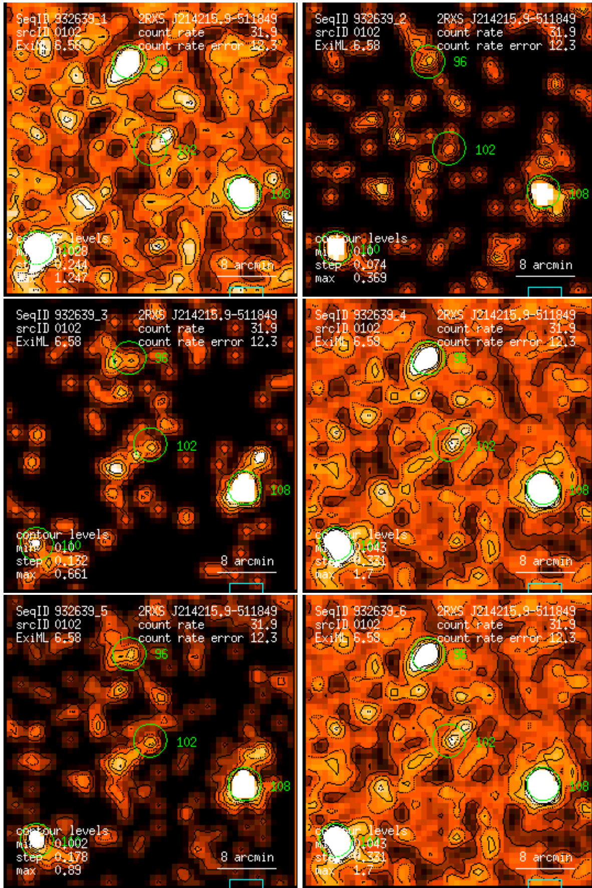
Figure 102: RASS 932639: detection 0102: band rate images, Gaussian filter: (1) PSPC channels 11 – 41, (2) 52 – 90, (3) 91 – 201, (4) 11 – 235, (5) 52 – 201, (6) 11 – 201. Broad band rates in counts/ks. Band rate contour levels in counts/ks/arcmin 2 .
