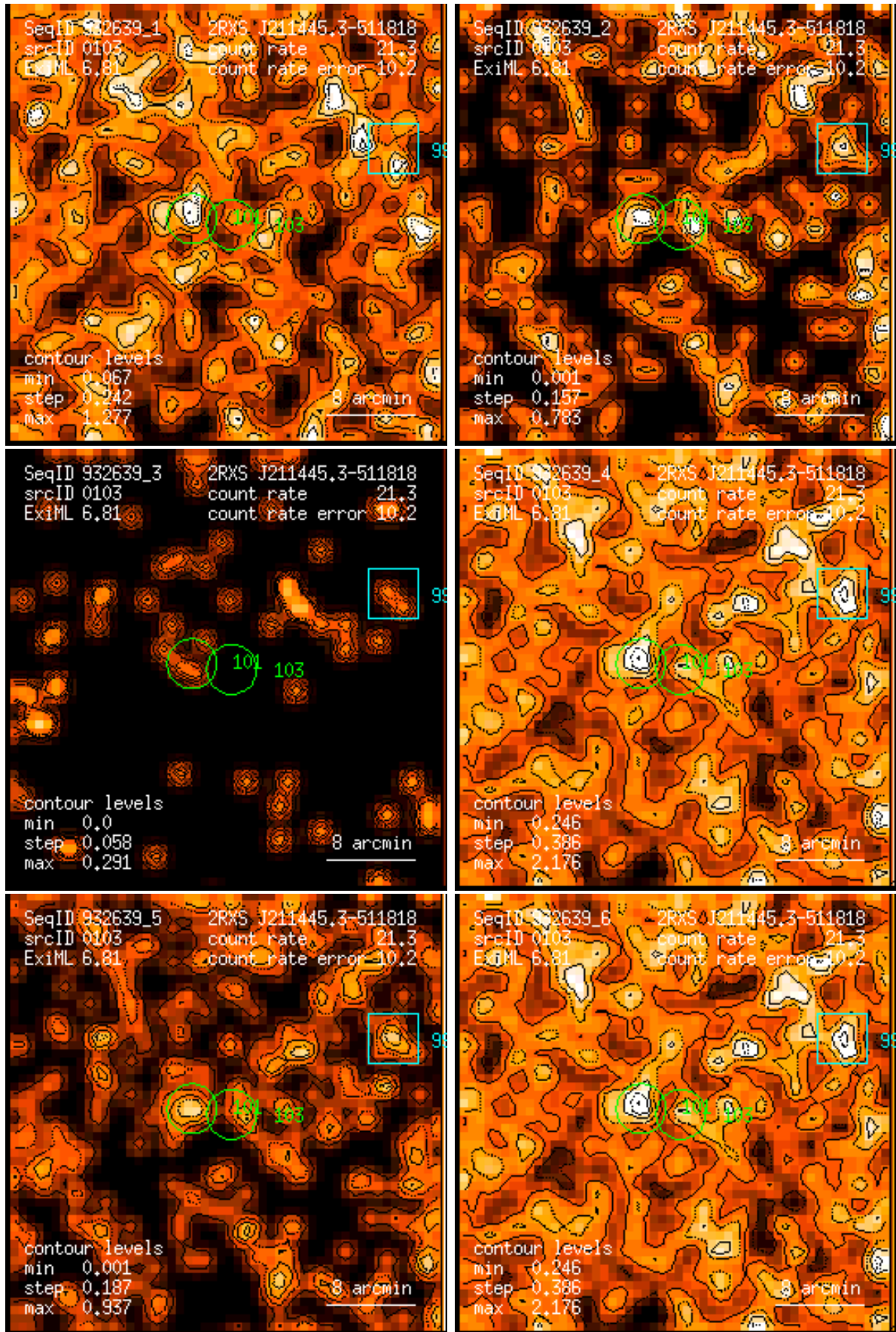
Figure 103: RASS 932639: detection 0103: band rate images, Gaussian filter: (1) PSPC channels 11 – 41, (2) 52 – 90, (3) 91 – 201, (4) 11 – 235, (5) 52 – 201, (6) 11 – 201. Broad band rates in counts/ks. Band rate contour levels in counts/ks/arcmin 2 .
