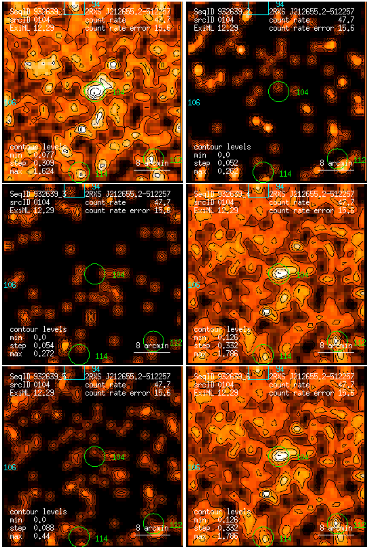
Figure 104: RASS 932639: detection 0104: band rate images, Gaussian filter: (1) PSPC channels 11 – 41, (2) 52 – 90, (3) 91 – 201, (4) 11 – 235, (5) 52 – 201, (6) 11 – 201. Broad band rates in counts/ks. Band rate contour levels in counts/ks/arcmin 2 .
