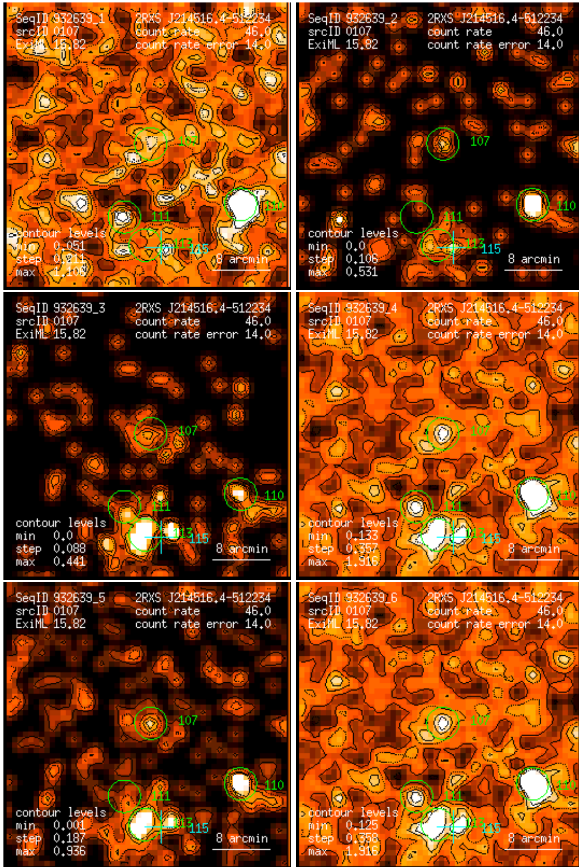
Figure 107: RASS 932639: detection 0107: band rate images, Gaussian filter: (1) PSPC channels 11 – 41, (2) 52 – 90, (3) 91 – 201, (4) 11 – 235, (5) 52 – 201, (6) 11 – 201. Broad band rates in counts/ks. Band rate contour levels in counts/ks/arcmin 2 .
