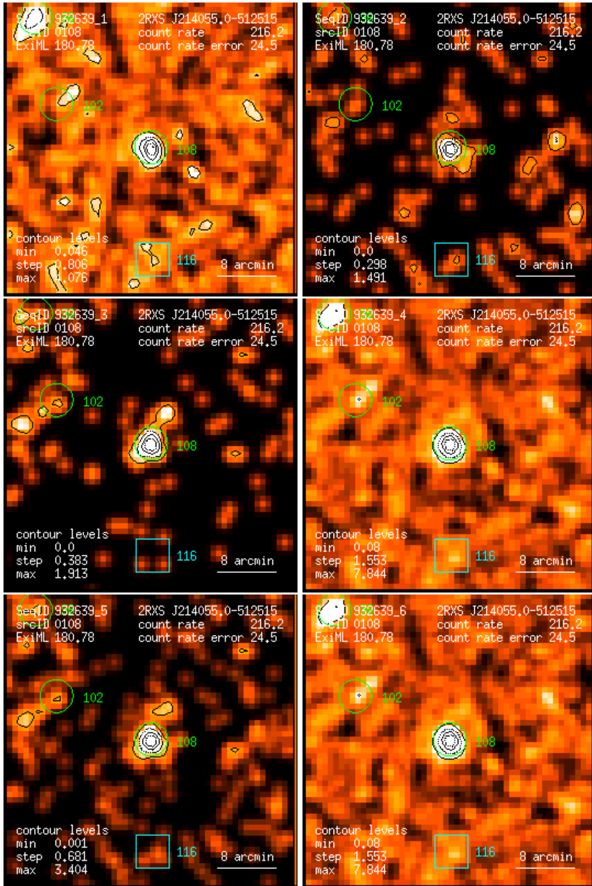
Figure 108: RASS 932639: detection 0108: band rate images, Gaussian filter: (1) PSPC channels 11 – 41, (2) 52 – 90, (3) 91 – 201, (4) 11 – 235, (5) 52 – 201, (6) 11 – 201. Broad band rates in counts/ks. Band rate contour levels in counts/ks/arcmin 2 .
