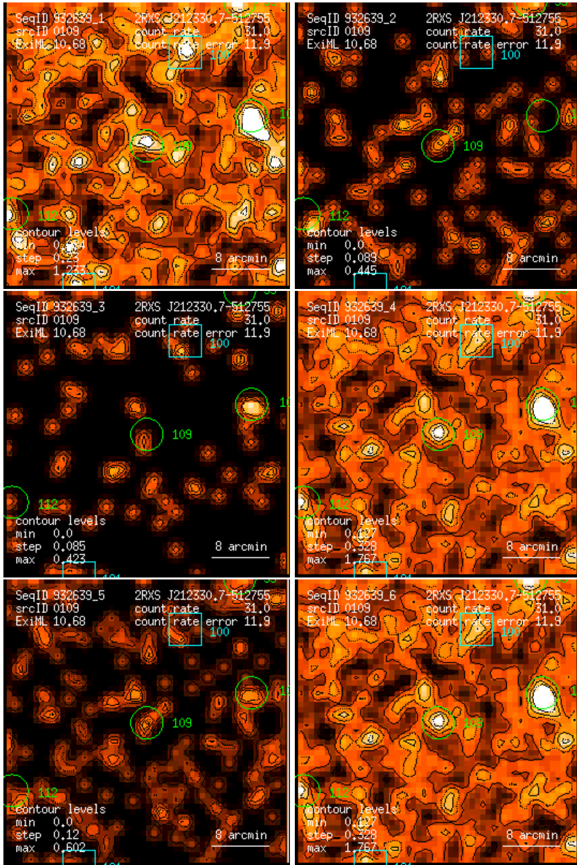
Figure 109: RASS 932639: detection 0109: band rate images, Gaussian filter: (1) PSPC channels 11 – 41, (2) 52 – 90, (3) 91 – 201, (4) 11 – 235, (5) 52 – 201, (6) 11 – 201. Broad band rates in counts/ks. Band rate contour levels in counts/ks/arcmin 2 .
