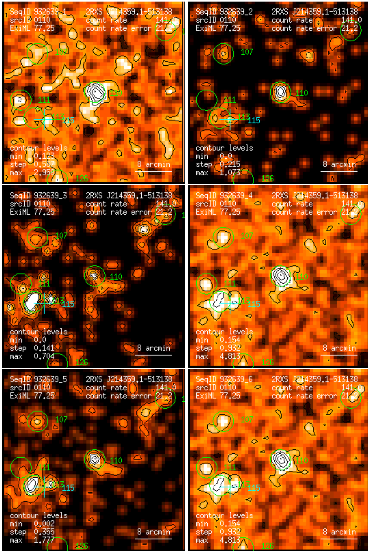
Figure 110: RASS 932639: detection 0110: band rate images, Gaussian filter: (1) PSPC channels 11 – 41, (2) 52 – 90, (3) 91 – 201, (4) 11 – 235, (5) 52 – 201, (6) 11 – 201. Broad band rates in counts/ks. Band rate contour levels in counts/ks/arcmin 2 .
