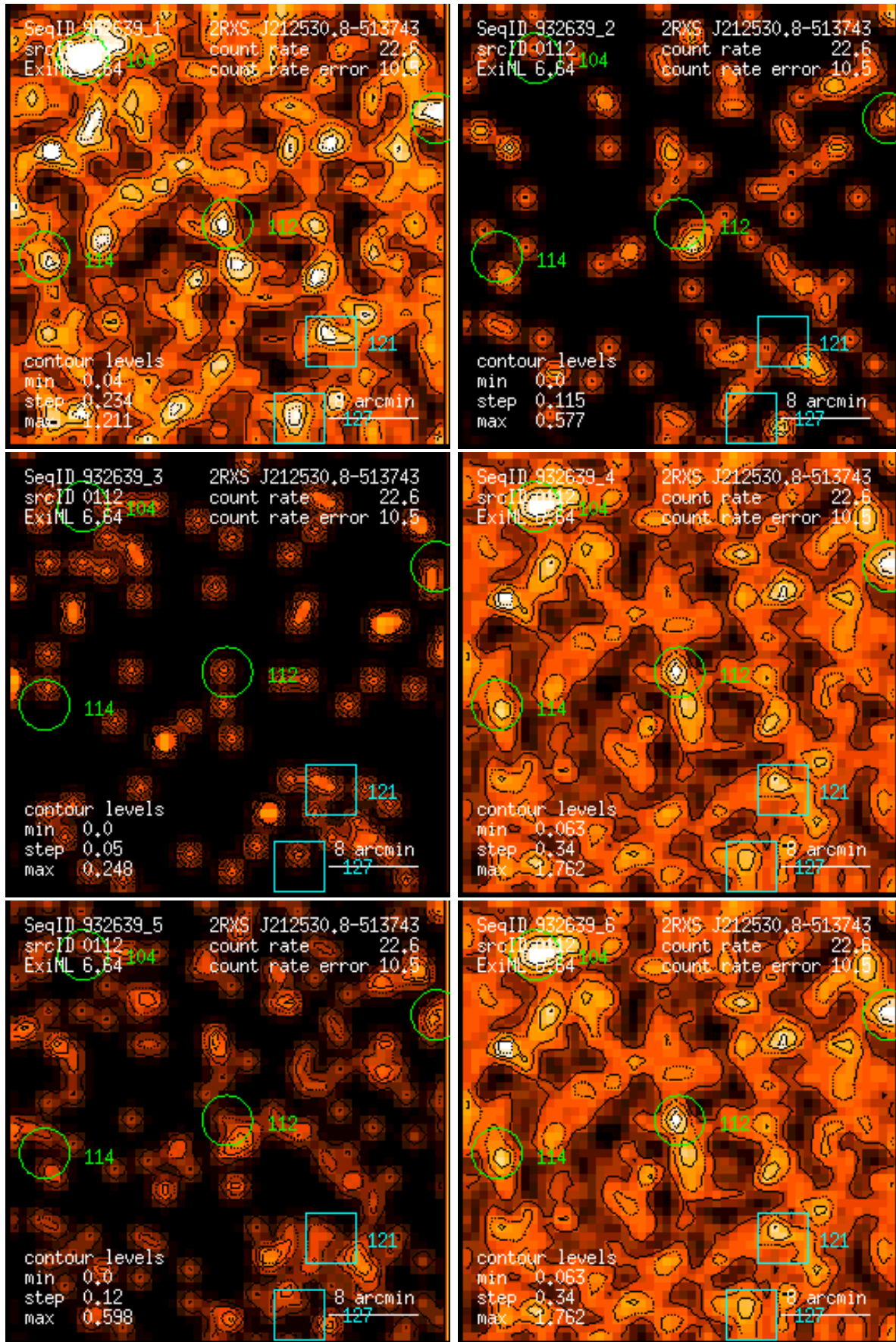
Figure 112: RASS 932639: detection 0112: band rate images, Gaussian filter: (1) PSPC channels 11 – 41, (2) 52 – 90, (3) 91 – 201, (4) 11 – 235, (5) 52 – 201, (6) 11 – 201. Broad band rates in counts/ks. Band rate contour levels in counts/ks/arcmin 2 .
