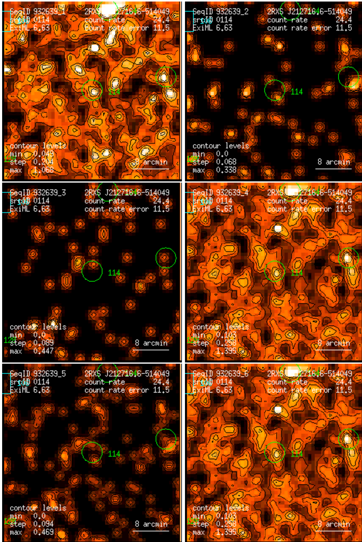
Figure 114: RASS 932639: detection 0114: band rate images, Gaussian filter: (1) PSPPC channels 11 – 41, (2) 52 – 90, (3) 91 – 201, (4) 11 – 235, (5) 52 – 201, (6) 11 – 201. Broad band rates in counts/ks. Band rate contour levels in counts/ks/arcmin 2 .
