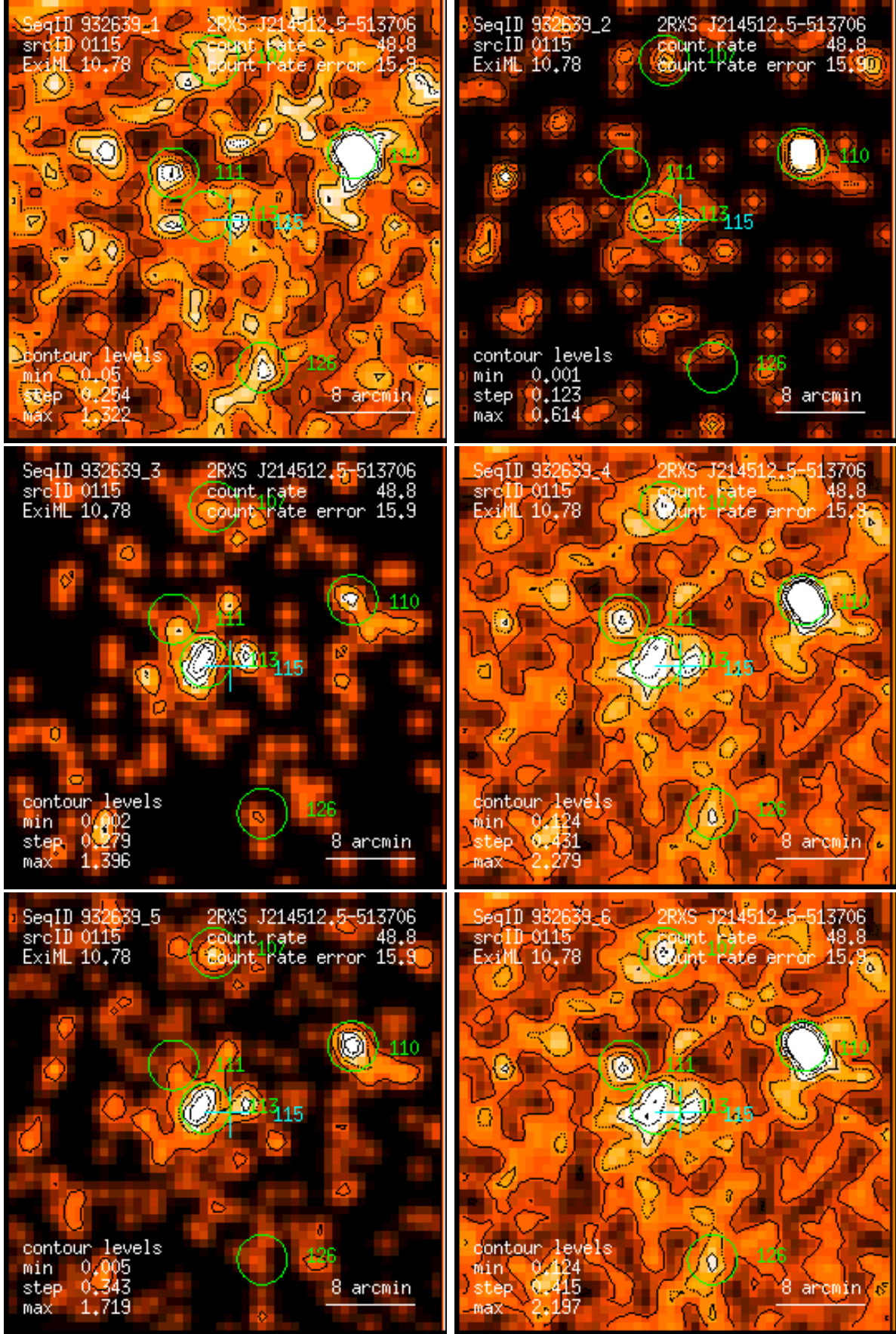
Figure 115: RASS 932639: detection 0115: band rate images, Gaussian filter: (1) PSPC channels 11 – 41, (2) 52 – 90, (3) 91 – 201, (4) 11 – 235, (5) 52 – 201, (6) 11 – 201. Broad band rates in counts/ks. Band rate contour levels in counts/ks/arcmin 2 .
