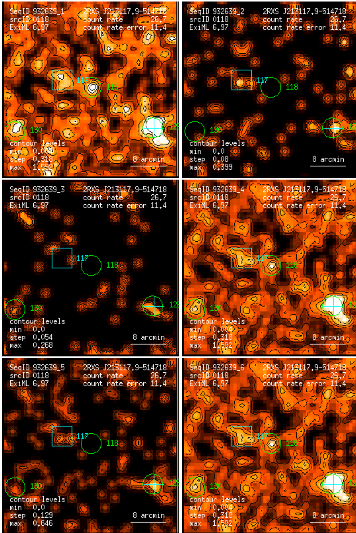
Figure 118: RASS 932639: detection 0118: band rate images, Gaussian filter: (1) PSPC channels 11 – 41, (2) 52 – 90, (3) 91 – 201, (4) 11 – 235, (5) 52 – 201, (6) 11 – 201. Broad band rates in counts/ks. Band rate contour levels in counts/ks/arcmin 2 .
