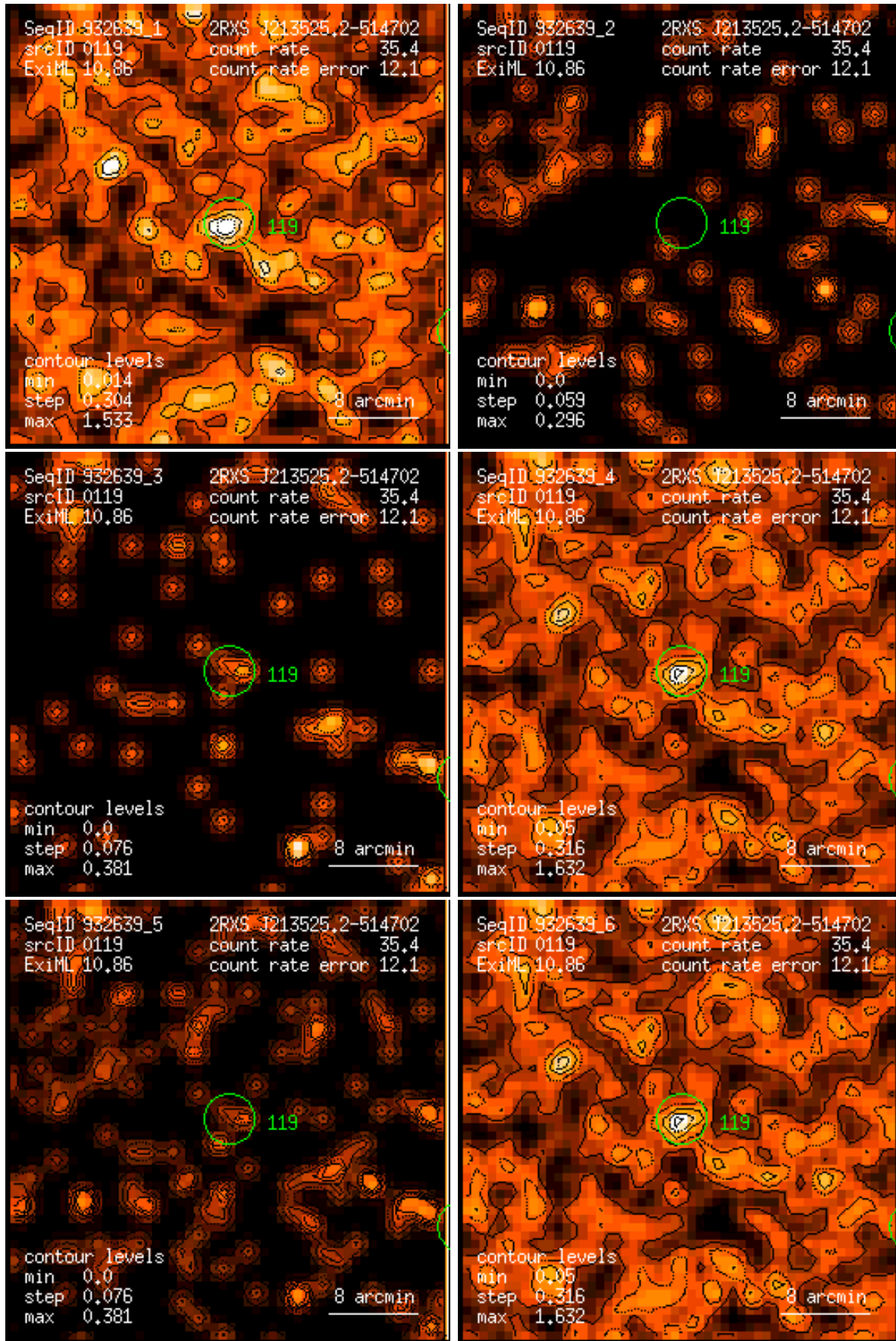
Figure 119: RASS 932639: detection 0119: band rate images, Gaussian filter: (1) PSPC channels 11 – 41, (2) 52 – 90, (3) 91 – 201, (4) 11 – 235, (5) 52 – 201, (6) 11 – 201. Broad band rates in counts/ks. Band rate contour levels in counts/ks/arcmin 2 .
