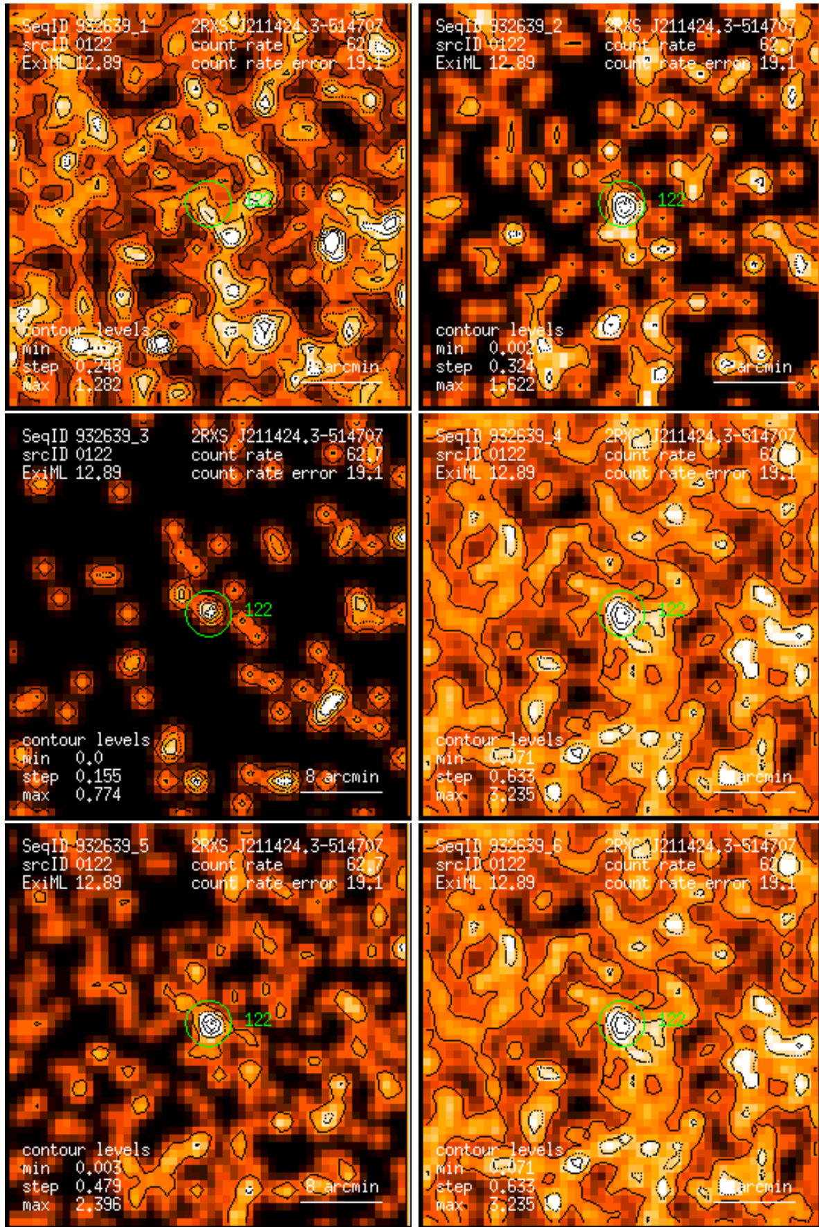
Figure 122: RASS 932639: detection 0122: band rate images, Gaussian filter: (1) PSPC channels 11 – 41, (2) 52 – 90, (3) 91 – 201, (4) 11 – 235, (5) 52 – 201, (6) 11 – 201. Broad band rates in counts/ks. Band rate contour levels in counts/ks/arcmin 2 .
