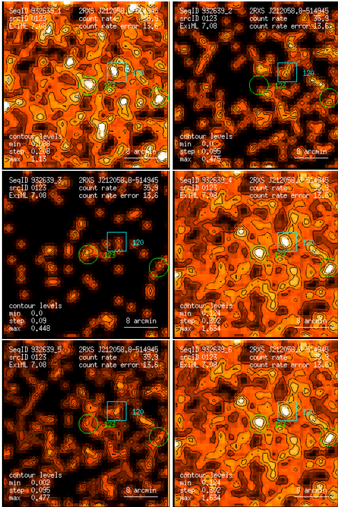
Figure 123: RASS 932639: detection 0123: band rate images, Gaussian filter: (1) PSPC channels 11 – 41, (2) 52 – 90, (3) 91 – 201, (4) 11 – 235, (5) 52 – 201, (6) 11 – 201. Broad band rates in counts/ks. Band rate contour levels in counts/ks/arcmin 2 .
