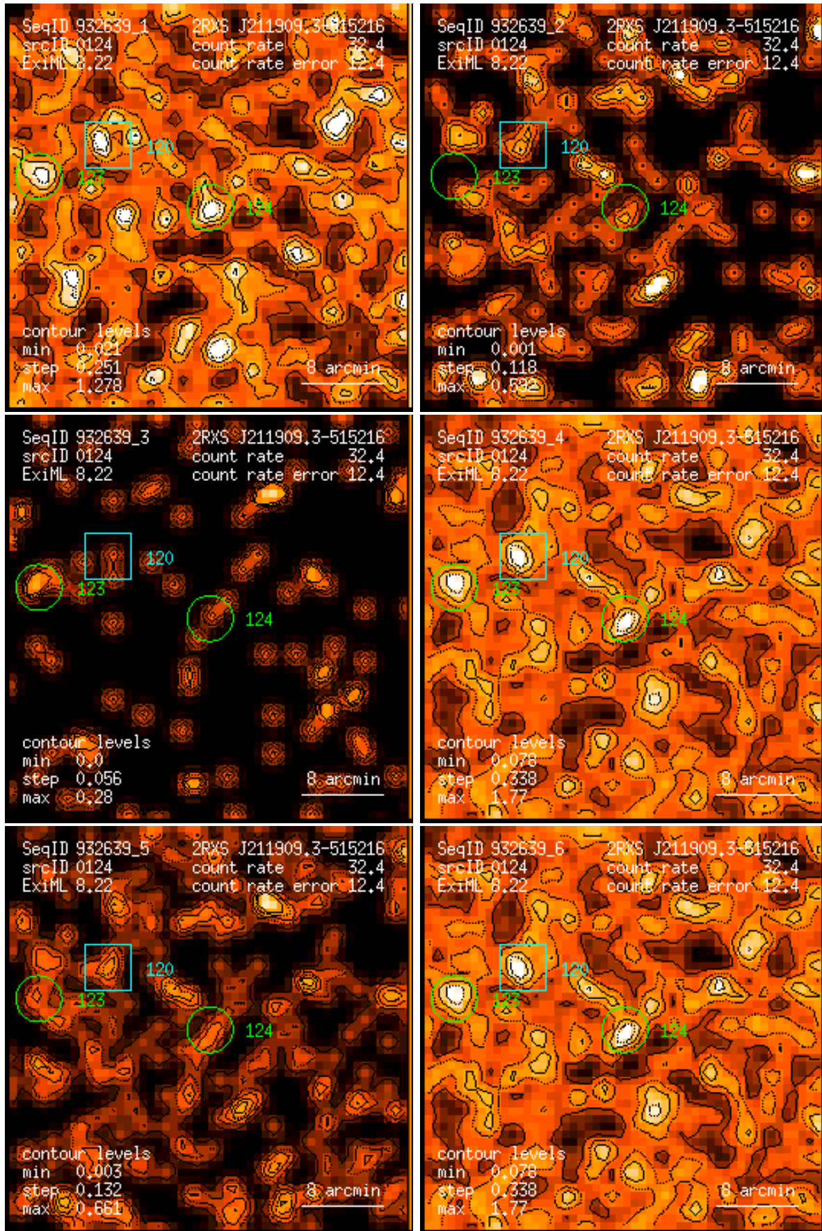
Figure 124: RASS 932639: detection 0124: band rate images, Gaussian filter: (1) PSPC channels 11 – 41, (2) 52 – 90, (3) 91 – 201, (4) 11 – 235, (5) 52 – 201, (6) 11 – 201. Broad band rates in counts/ks. Band rate contour levels in counts/ks/arcmin 2 .
