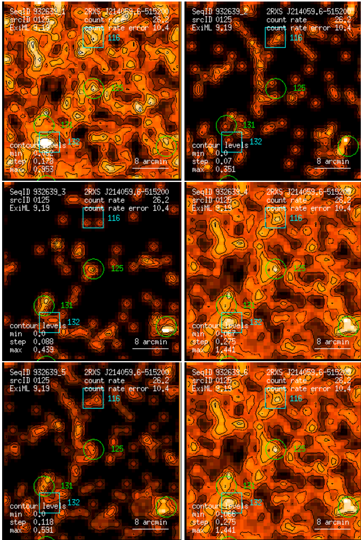
Figure 125: RASS 932639: detection 0125: band rate images, Gaussian filter: (1) PSPC channels 11 – 41, (2) 52 – 90, (3) 91 – 201, (4) 11 – 235, (5) 52 – 201, (6) 11 – 201. Broad band rates in counts/ks. Band rate contour levels in counts/ks/arcmin 2 .
