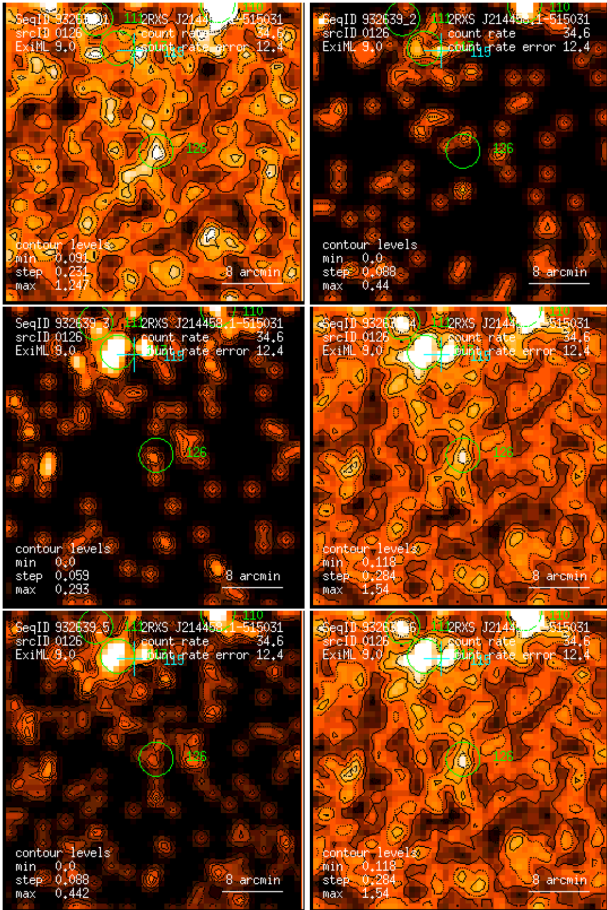
Figure 126: RASS 932639: detection 0126: band rate images, Gaussian filter: (1) PSPC channels 11 – 41, (2) 52 – 90, (3) 91 – 201, (4) 11 – 235, (5) 52 – 201, (6) 11 – 201. Broad band rates in counts/ks. Band rate contour levels in counts/ks/arcmin 2 .
