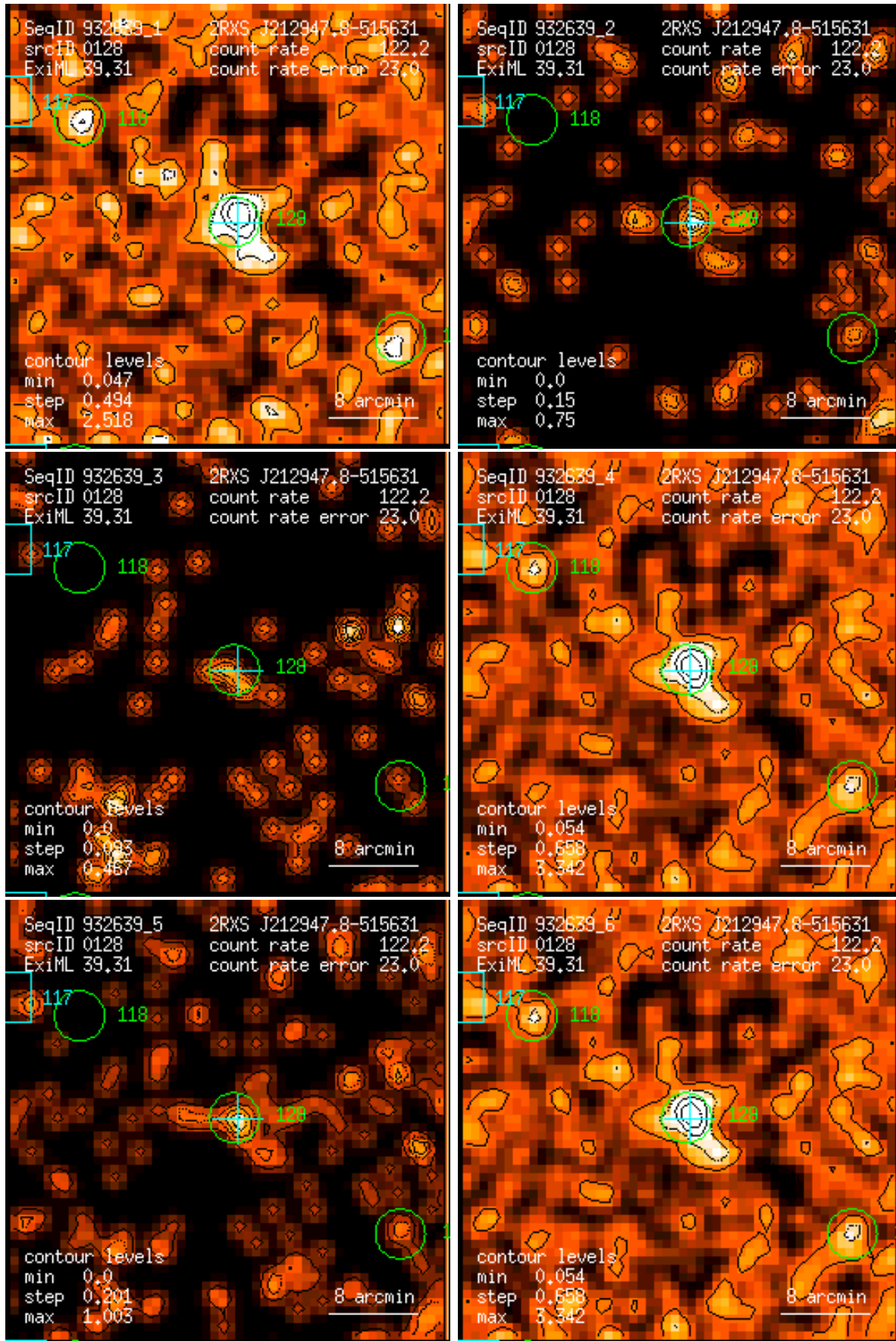
Figure 128: RASS 932639: detection 0128: band rate images, Gaussian filter: (1) PSPC channels 11 – 41, (2) 52 – 90, (3) 91 – 201, (4) 11 – 235, (5) 52 – 201, (6) 11 – 201. Broad band rates in counts/ks. Band rate contour levels in counts/ks/arcmin 2 .
