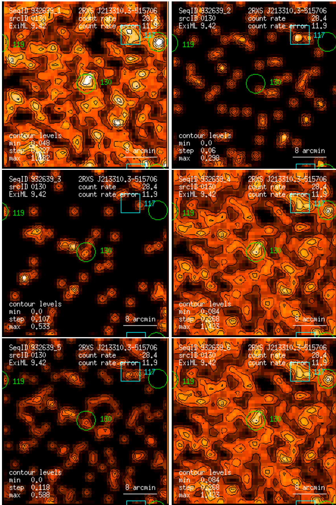
Figure 130: RASS 932639: detection 0130: band rate images, Gaussian filter: (1) PSPC channels 11 – 41, (2) 52 – 90, (3) 91 – 201, (4) 11 – 235, (5) 52 – 201, (6) 11 – 201. Broad band rates in counts/ks. Band rate contour levels in counts/ks/arcmin 2 .
