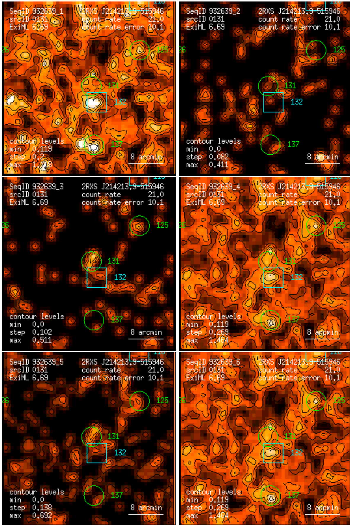
Figure 131: RASS 932639: detection 0131: band rate images, Gaussian filter: (1) PSPC channels 11 – 41, (2) 52 – 90, (3) 91 – 201, (4) 11 – 235, (5) 52 – 201, (6) 11 – 201. Broad band rates in counts/ks. Band rate contour levels in counts/ks/arcmin 2 .
