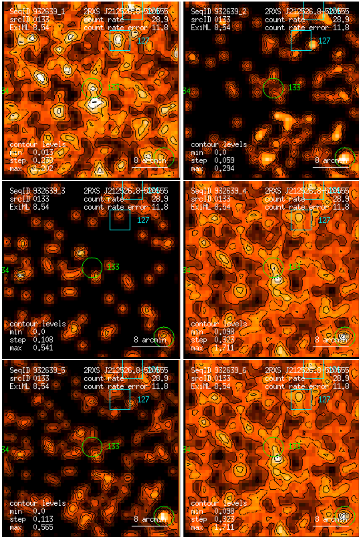
Figure 133: RASS 932639: detection 0133: band rate images, Gaussian filter: (1) PSPC channels 11 – 41, (2) 52 – 90, (3) 91 – 201, (4) 11 – 235, (5) 52 – 201, (6) 11 – 201. Broad band rates in counts/ks. Band rate contour levels in counts/ks/arcmin 2 .
