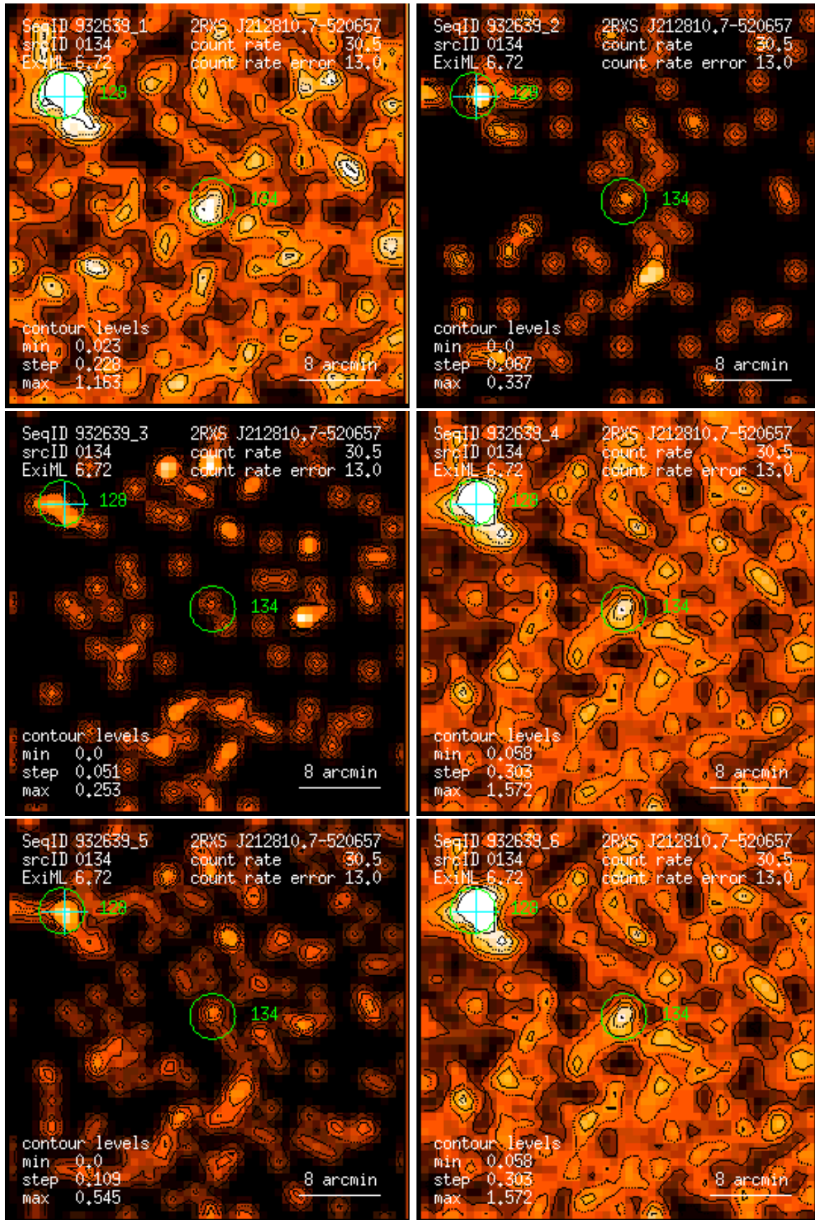
Figure 134: RASS 932639: detection 0134: band rate images, Gaussian filter: (1) PSPC channels 11 – 41, (2) 52 – 90, (3) 91 – 201, (4) 11 – 235, (5) 52 – 201, (6) 11 – 201. Broad band rates in counts/ks. Band rate contour levels in counts/ks/arcmin 2 .
