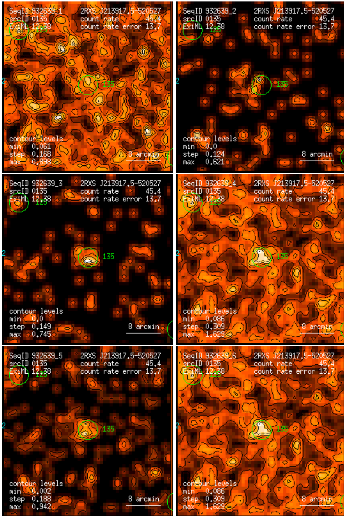
Figure 135: RASS 932639: detection 0135: band rate images, Gaussian filter: (1) PSPC channels 11 – 41, (2) 52 – 90, (3) 91 – 201, (4) 11 – 235, (5) 52 – 201, (6) 11 – 201. Broad band rates in counts/ks. Band rate contour levels in counts/ks/arcmin 2 .
