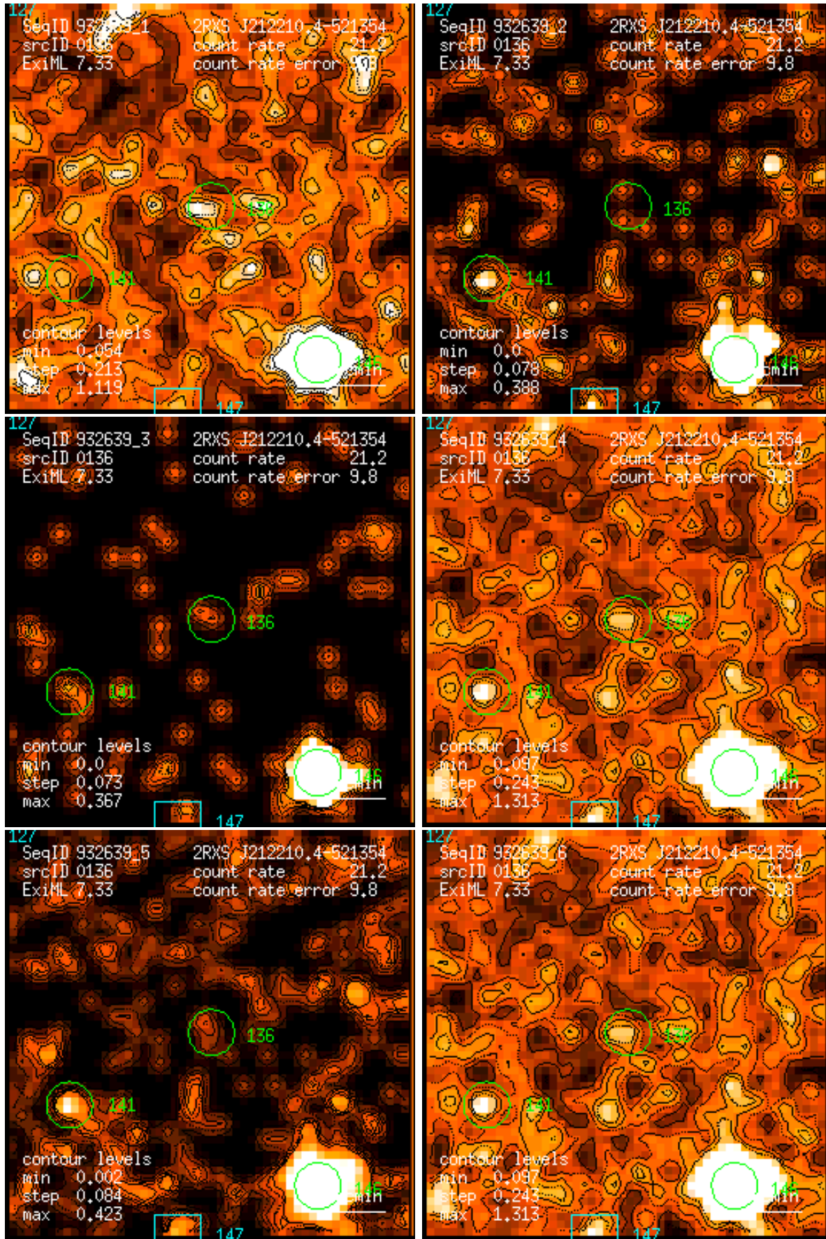
Figure 136: RASS 932639: detection 0136: band rate images, Gaussian filter: (1) PSPC channels 11 – 41, (2) 52 – 90, (3) 91 – 201, (4) 11 – 235, (5) 52 – 201, (6) 11 – 201. Broad band rates in counts/ks. Band rate contour levels in counts/ks/arcmin 2 .
