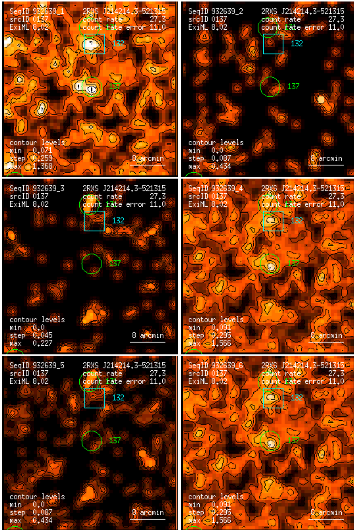
Figure 137: RASS 932639: detection 0137: band rate images, Gaussian filter: (1) PSPC channels 11 – 41, (2) 52 – 90, (3) 91 – 201, (4) 11 – 235, (5) 52 – 201, (6) 11 – 201. Broad band rates in counts/ks. Band rate contour levels in counts/ks/arcmin 2 .
