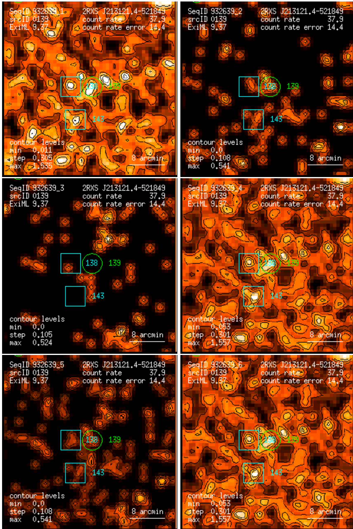
Figure 139: RASS 932639: detection 0139: band rate images, Gaussian filter: (1) PSPC channels 11 – 41, (2) 52 – 90, (3) 91 – 201, (4) 11 – 235, (5) 52 – 201, (6) 11 – 201. Broad band rates in counts/ks. Band rate contour levels in counts/ks/arcmin 2 .
