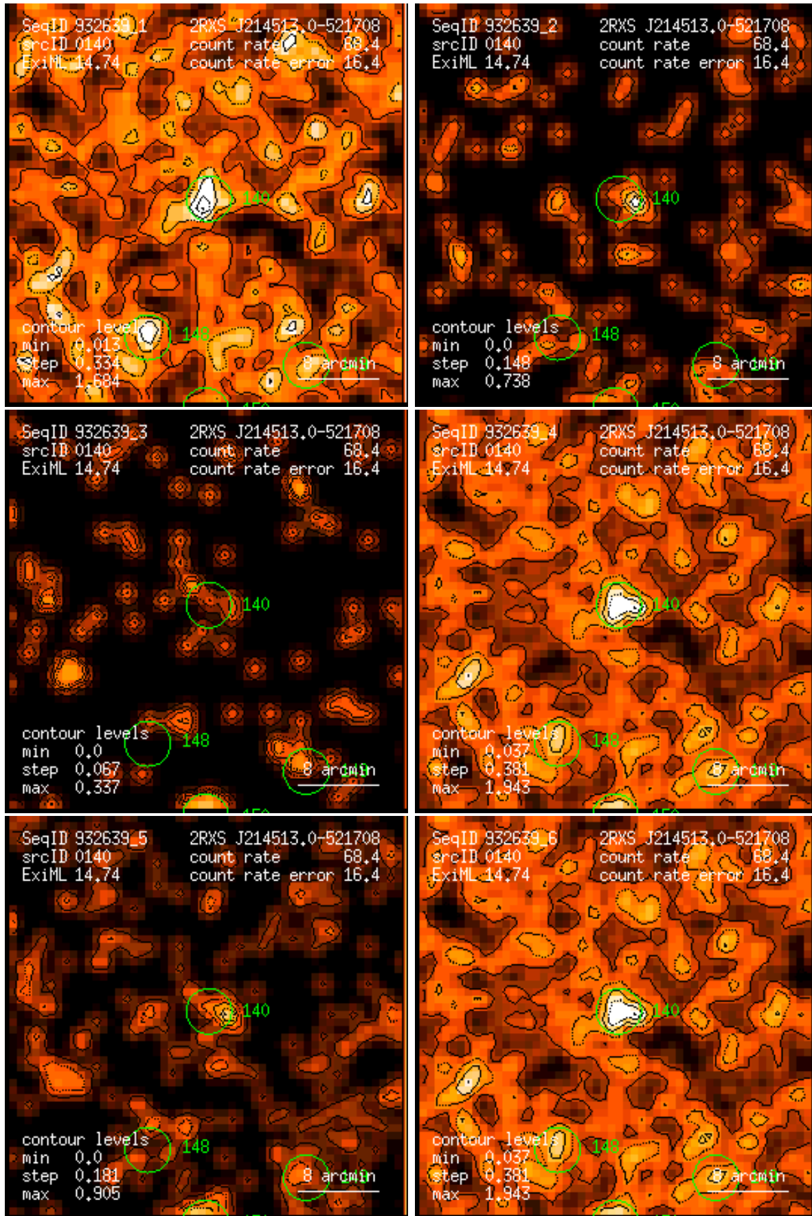
Figure 140: RASS 932639: detection 0140: band rate images, Gaussian filter: (1) PSPC channels 11 – 41, (2) 52 – 90, (3) 91 – 201, (4) 11 – 235, (5) 52 – 201, (6) 11 – 201. Broad band rates in counts/ks. Band rate contour levels in counts/ks/arcmin 2 .
