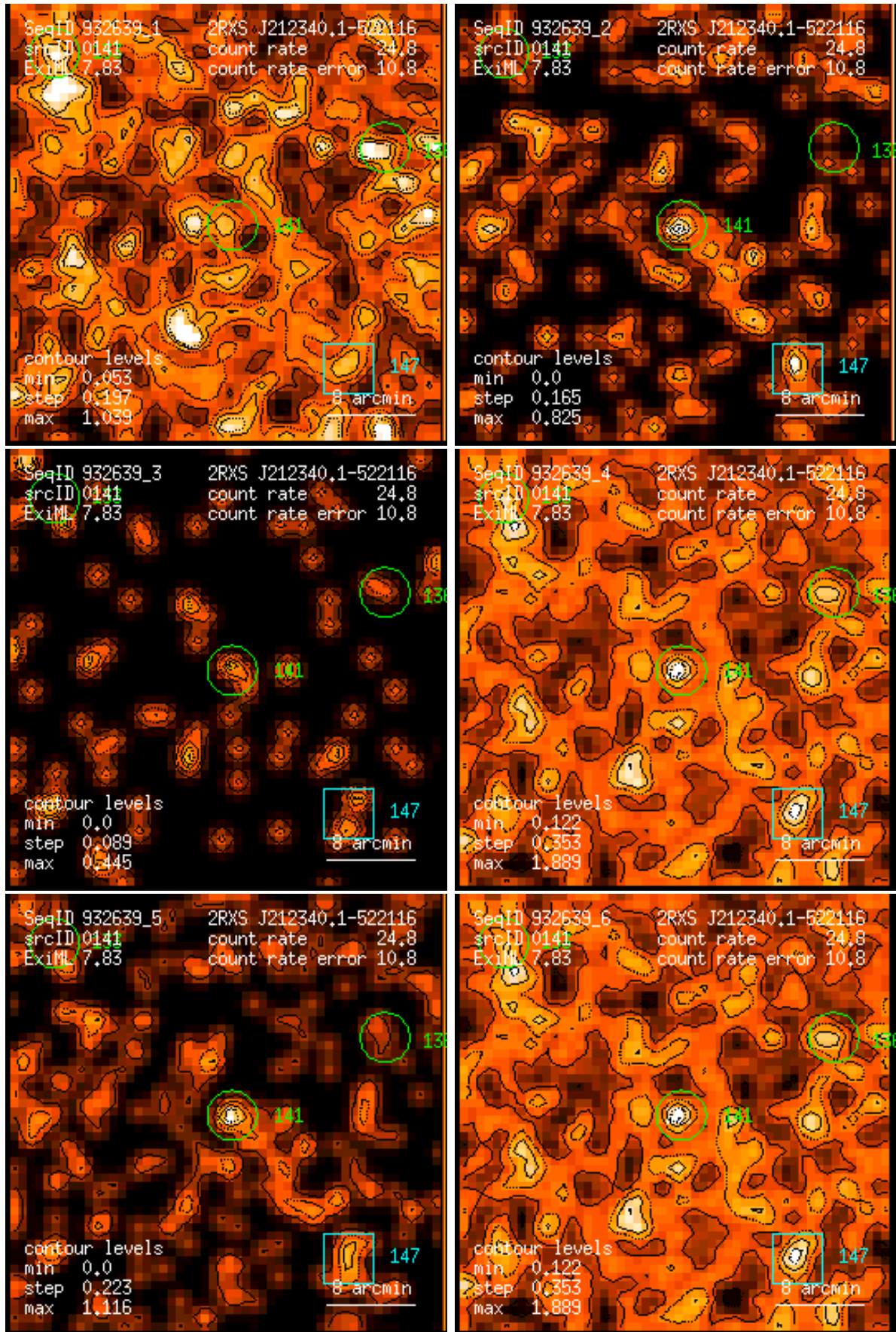
Figure 141: RASS 932639: detection 0141: band rate images, Gaussian filter: (1) PSPC channels 11 – 41, (2) 52 – 90, (3) 91 – 201, (4) 11 – 235, (5) 52 – 201, (6) 11 – 201. Broad band rates in counts/ks. Band rate contour levels in counts/ks/arcmin 2 .
