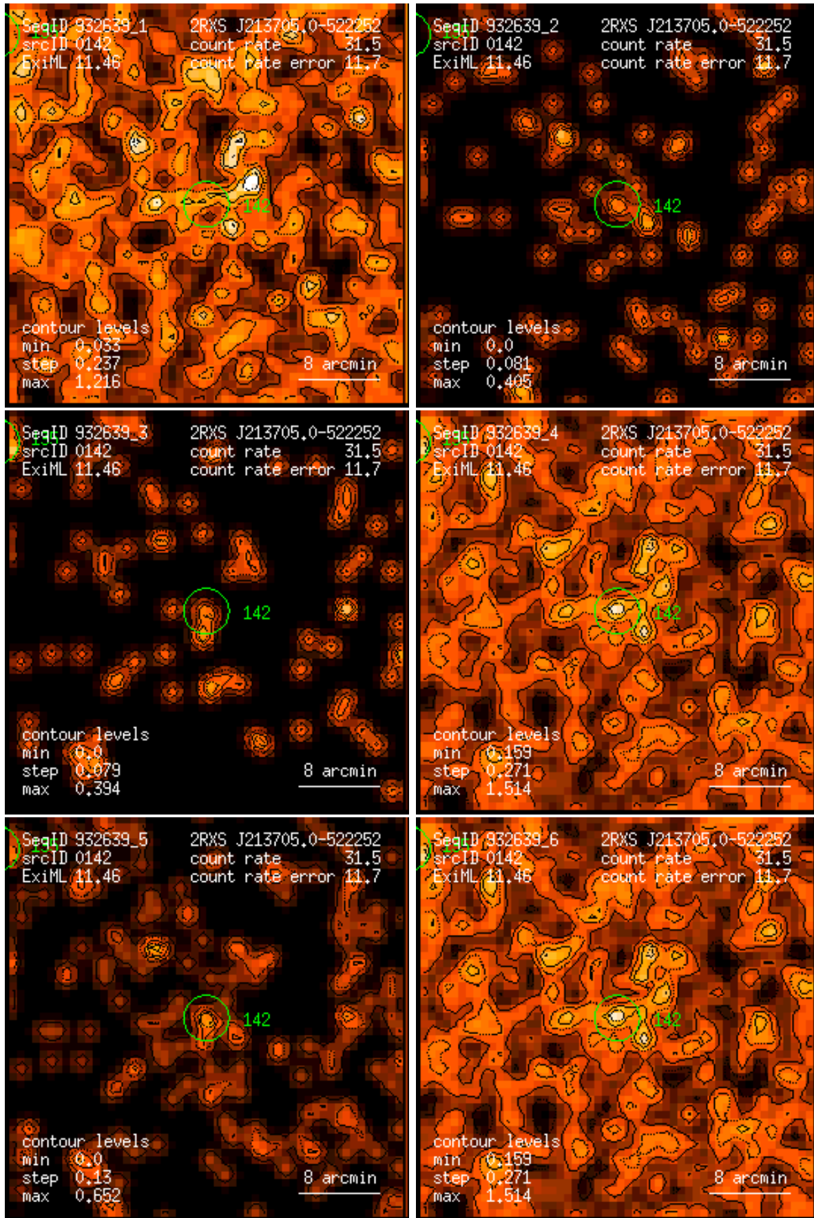
Figure 142: RASS 932639: detection 0142: band rate images, Gaussian filter: (1) PSPC channels 11 – 41, (2) 52 – 90, (3) 91 – 201, (4) 11 – 235, (5) 52 – 201, (6) 11 – 201. Broad band rates in counts/ks. Band rate contour levels in counts/ks/arcmin 2 .
