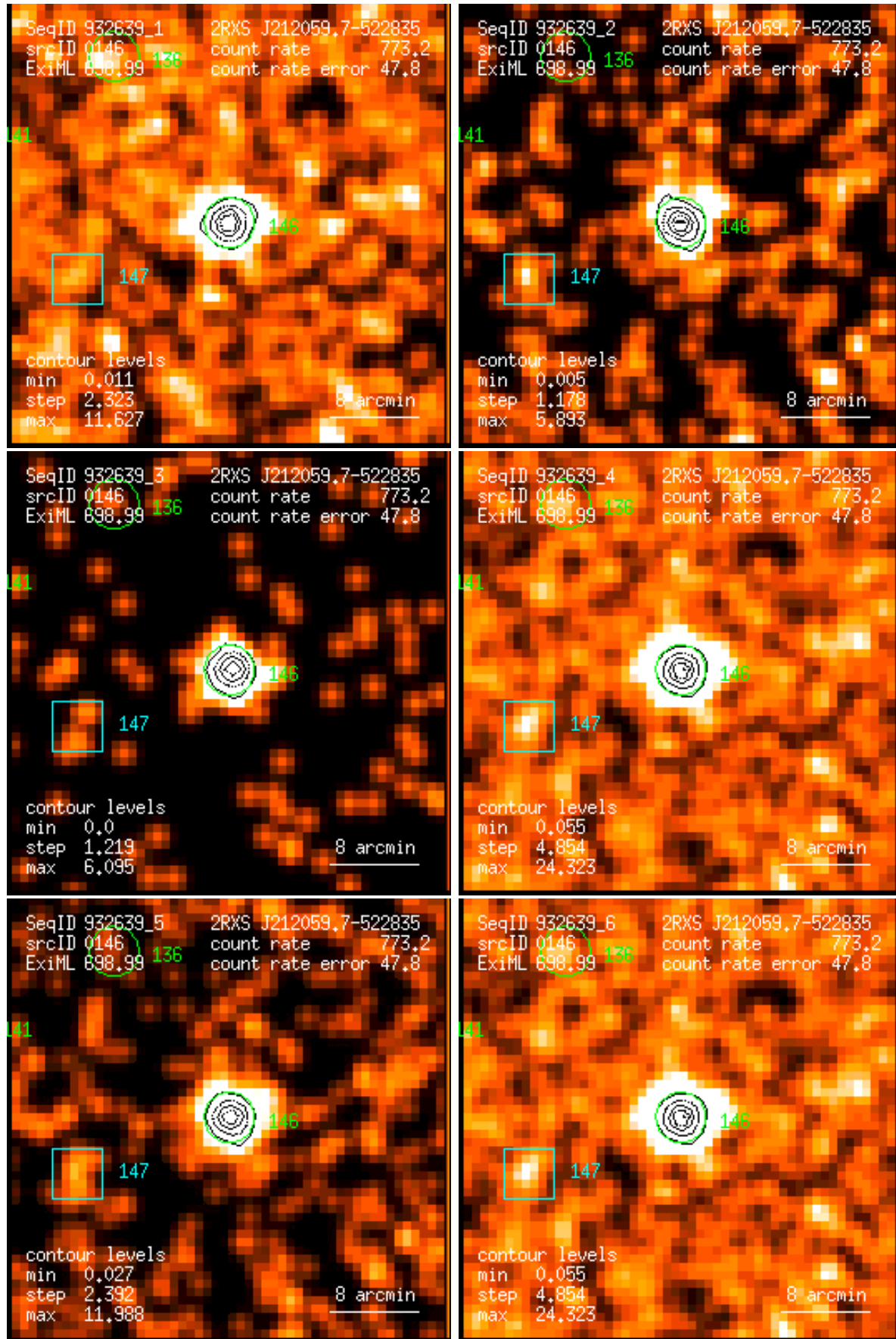
Figure 146: RASS 932639: detection 0146: band rate images, Gaussian filter: (1) PSPC channels 11 – 41, (2) 52 – 90, (3) 91 – 201, (4) 11 – 235, (5) 52 – 201, (6) 11 – 201. Broad band rates in counts/ks. Band rate contour levels in counts/ks/arcmin 2 .
