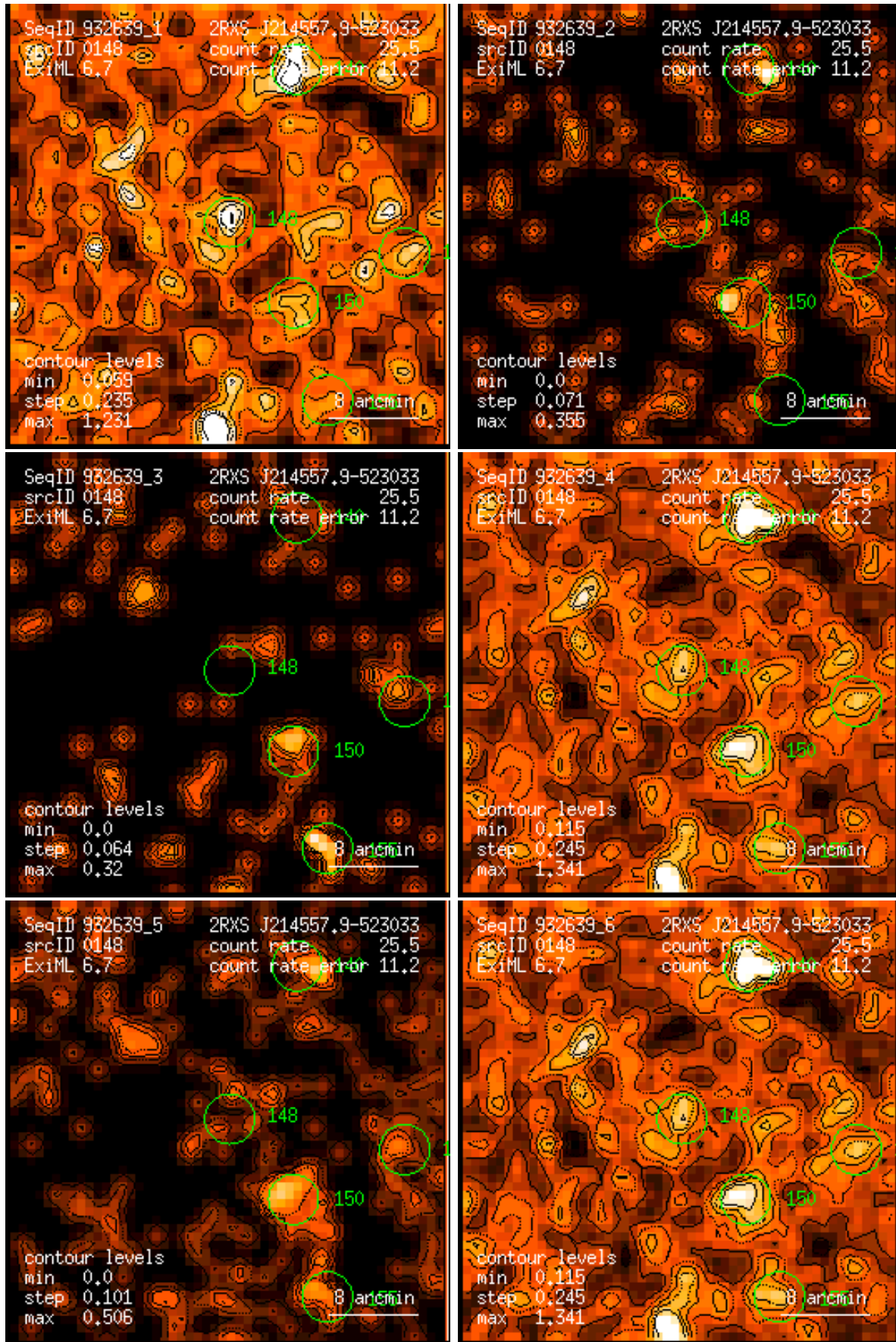
Figure 148: RASS 932639: detection 0148: band rate images, Gaussian filter: (1) PSPC channels 11 – 41, (2) 52 – 90, (3) 91 – 201, (4) 11 – 235, (5) 52 – 201, (6) 11 – 201. Broad band rates in counts/ks. Band rate contour levels in counts/ks/arcmin 2 .
