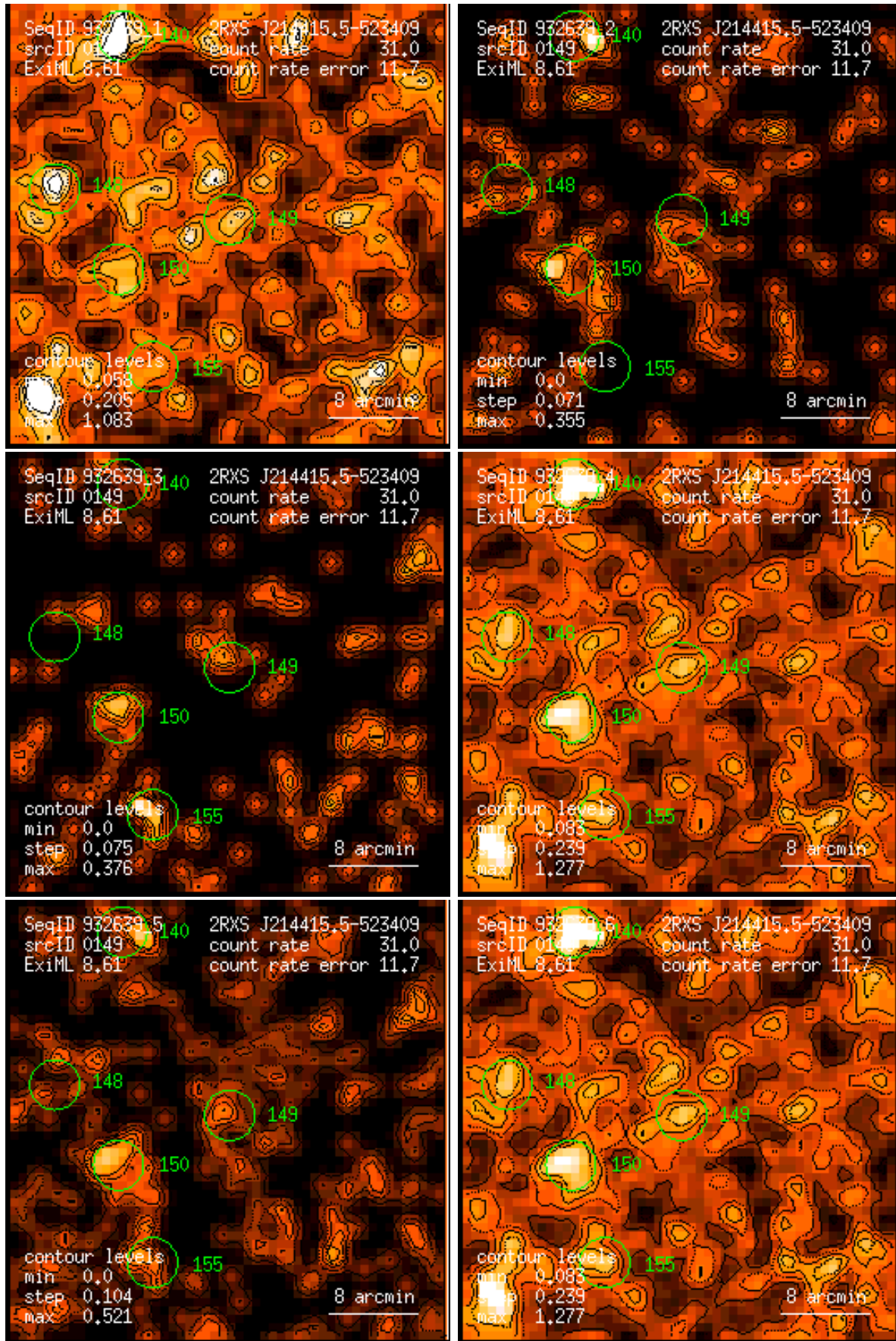
Figure 149: RASS 932639: detection 0149: band rate images, Gaussian filter: (1) PSPC channels 11 – 41, (2) 52 – 90, (3) 91 – 201, (4) 11 – 235, (5) 52 – 201, (6) 11 – 201. Broad band rates in counts/ks. Band rate contour levels in counts/ks/arcmin 2 .
