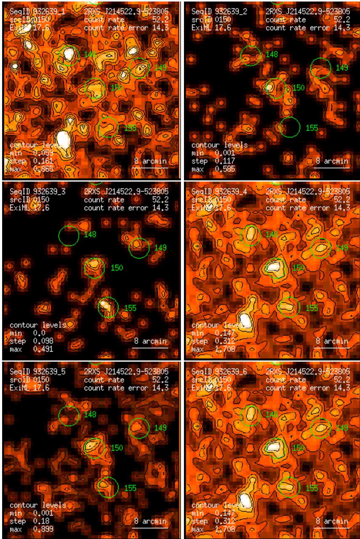
Figure 150: RASS 932639: detection 0150: band rate images, Gaussian filter: (1) PSPC channels 11 – 41, (2) 52 – 90, (3) 91 – 201, (4) 11 – 235, (5) 52 – 201, (6) 11 – 201. Broad band rates in counts/ks. Band rate contour levels in counts/ks/arcmin 2 .
