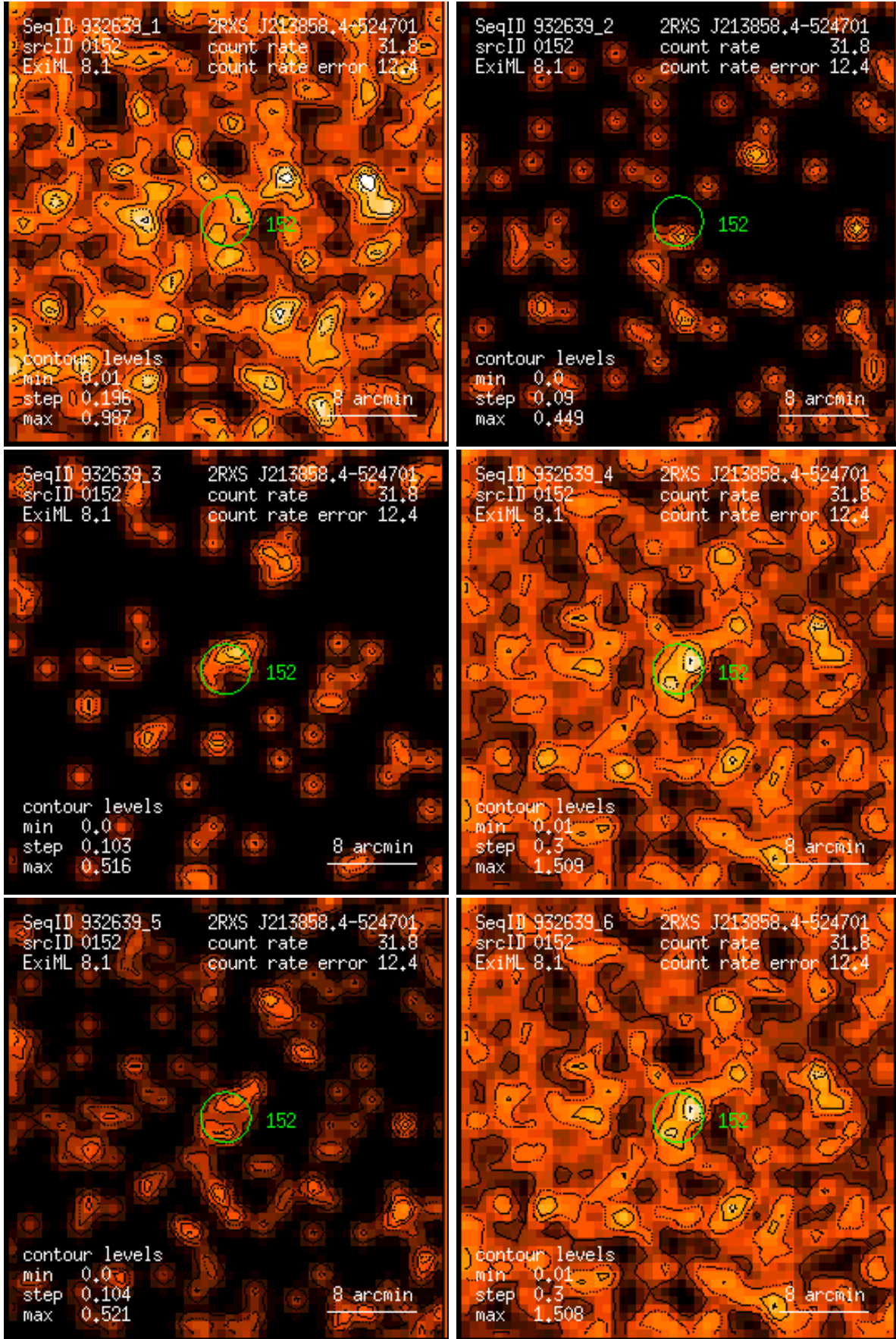
Figure 152: RASS 932639: detection 0152: band rate images, Gaussian filter: (1) PSPC channels 11 – 41, (2) 52 – 90, (3) 91 – 201, (4) 11 – 235, (5) 52 – 201, (6) 11 – 201. Broad band rates in counts/ks. Band rate contour levels in counts/ks/arcmin 2 .
